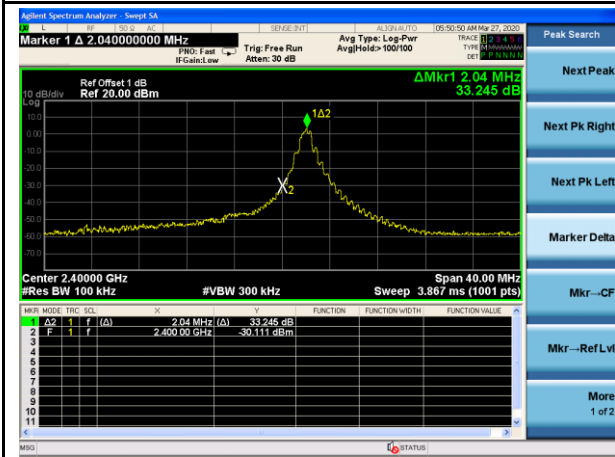
BLE-Band Edge-Low-2Mbps
