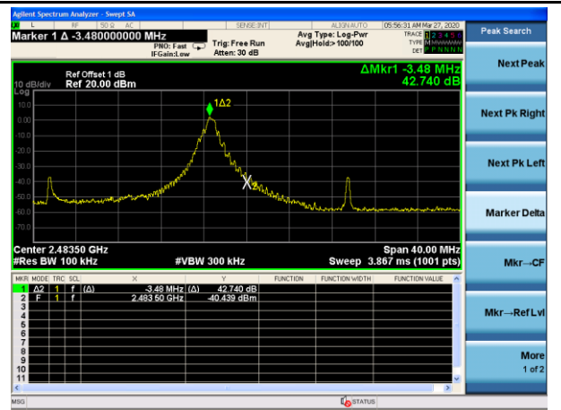
BLE-Band Edge-High-2Mbps
