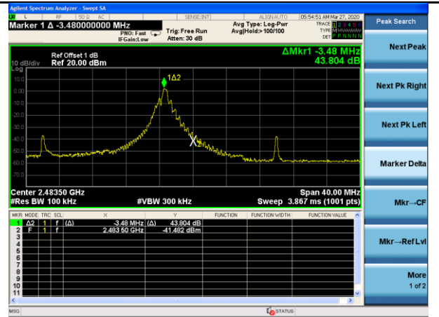
BLE-Band Edge-High-1Mbps
