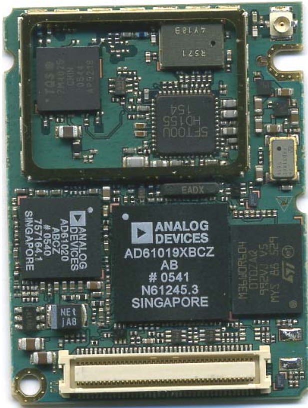
TC65: component side shielding opened
