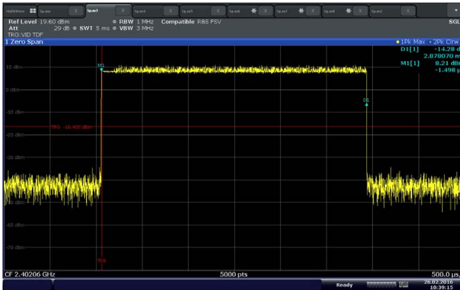
8DPSK width of single pulse (2.878 ms)
