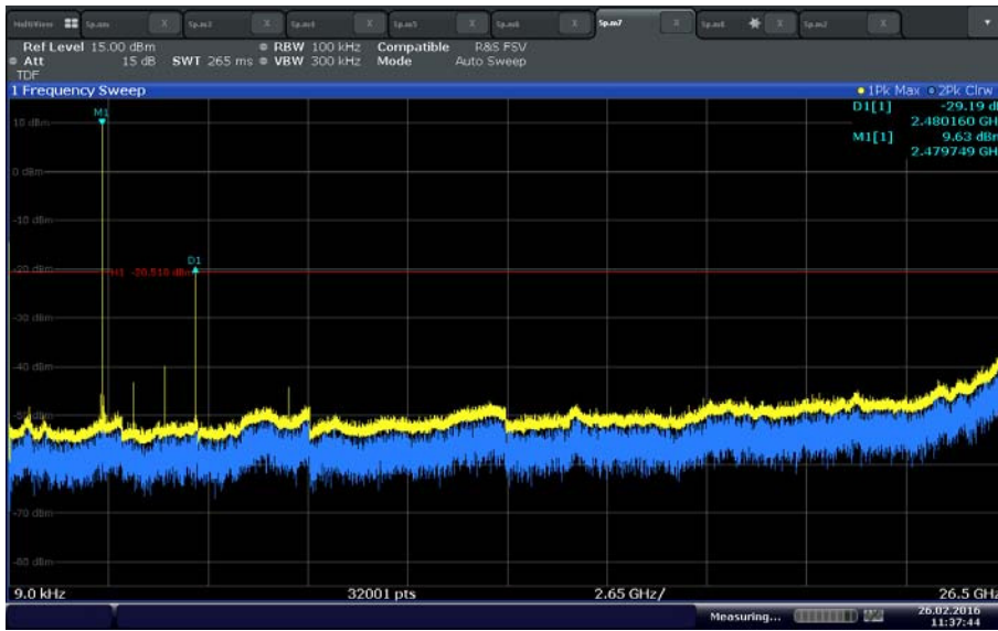
High Channel (GFSK) – 2 nd harmonic complies with 20dBc
