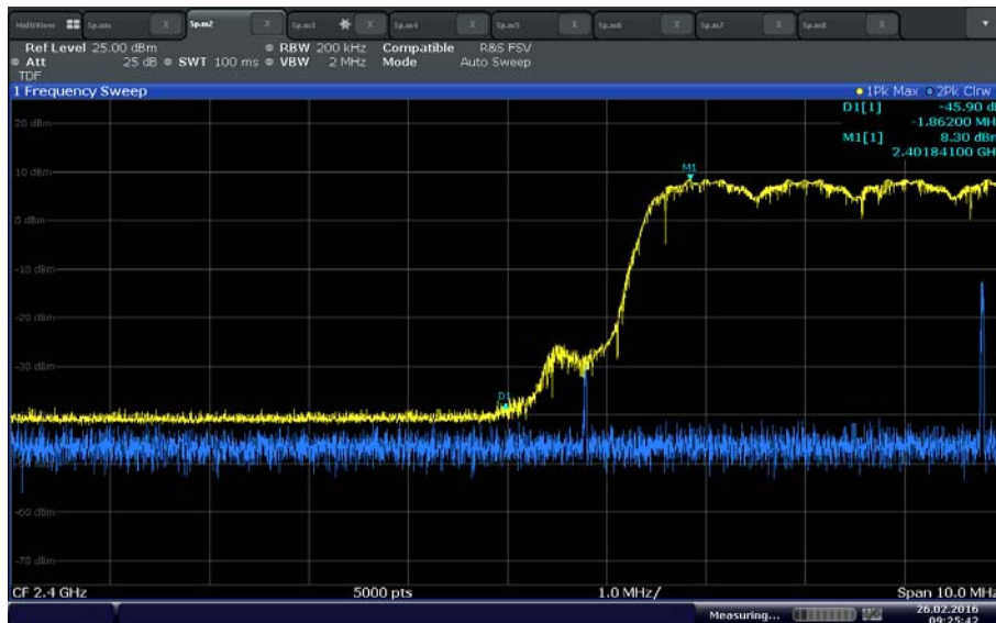
Hopping lower bandedge ( \pi/4 -DQPSK)
