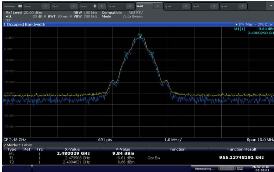
GFSK High Channel
