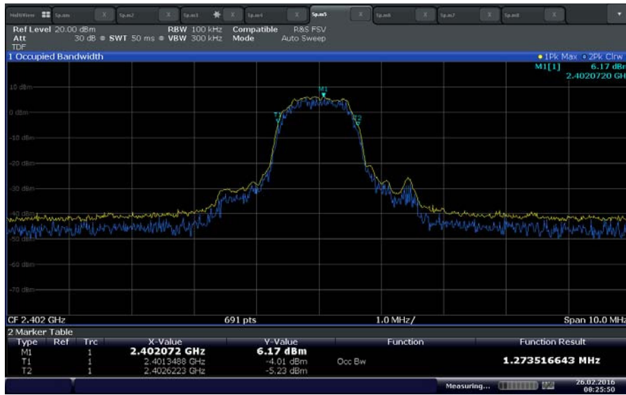
8DPSK Low Channel
