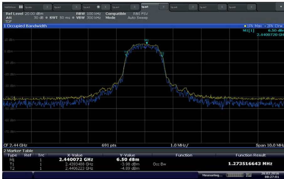
8DPSK Mid Channel
