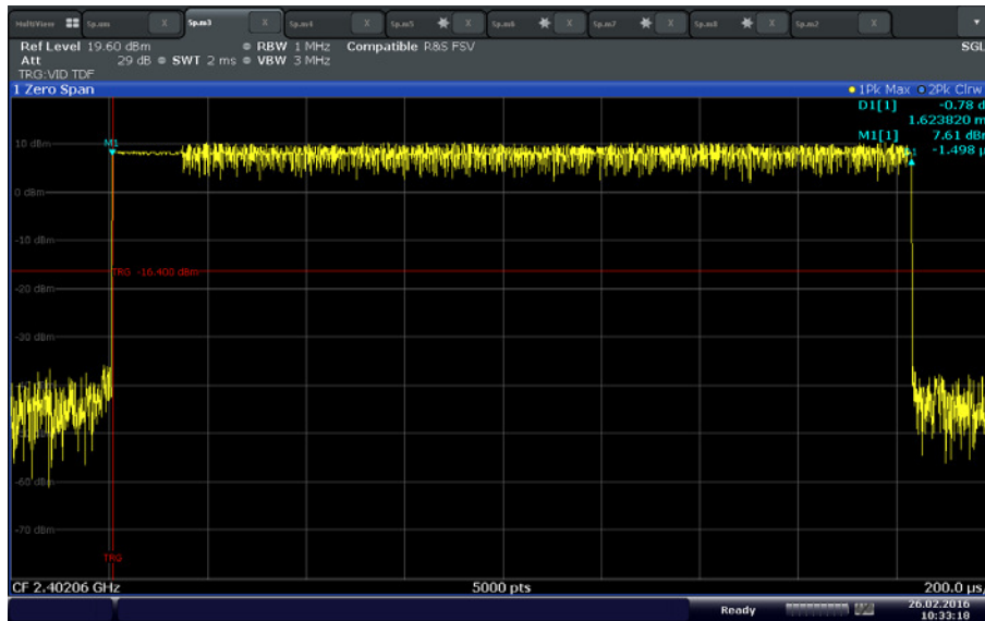
\pi/4 -DQPSK width of single pulse (1.6238 ms)
