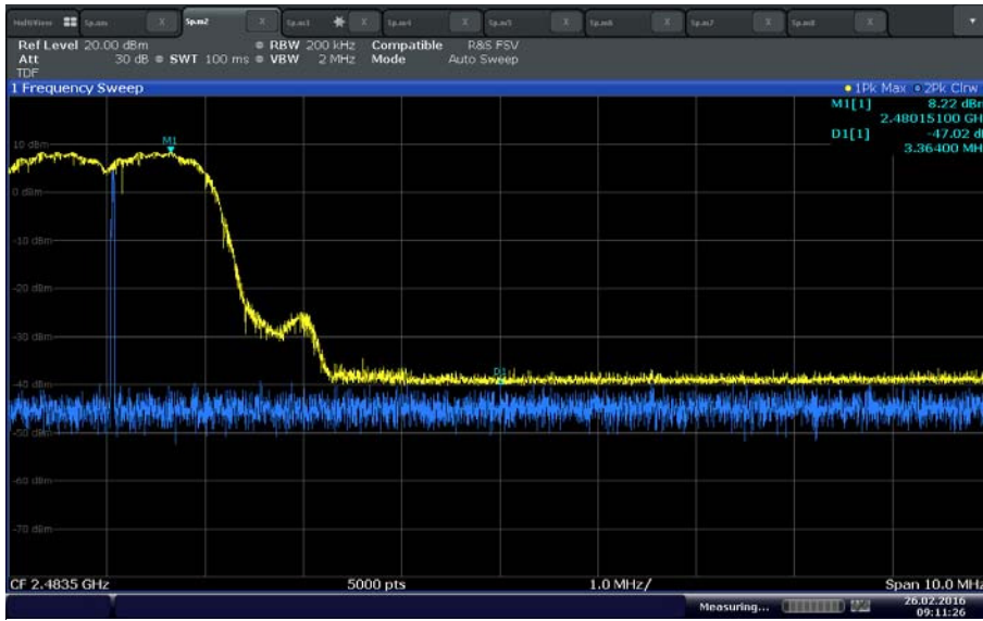
Hopping upper bandedge ( \pi/4 -DQPSK)
