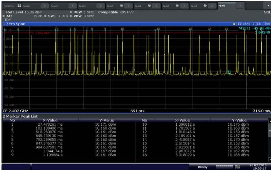
18 pulses/3.16 seconds (2-DH3)
