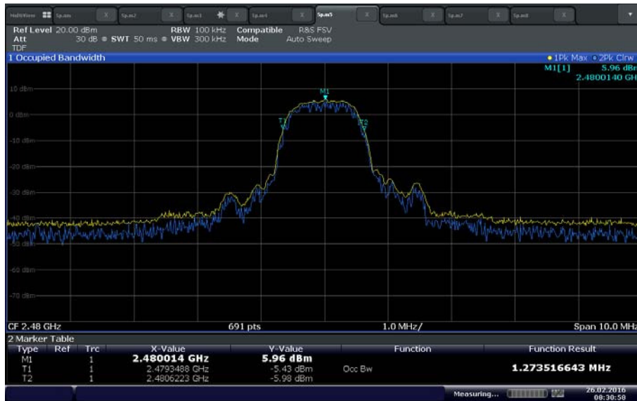
\pi/4 -DQPSK High Channel
