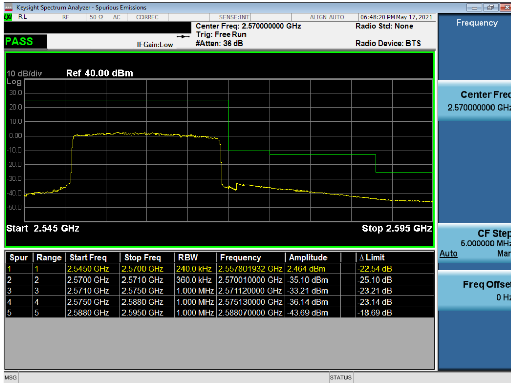
Plot 7-19. Upper ACP Plot (LTE Band 7 - 20MHz QPSK – Full RB)
