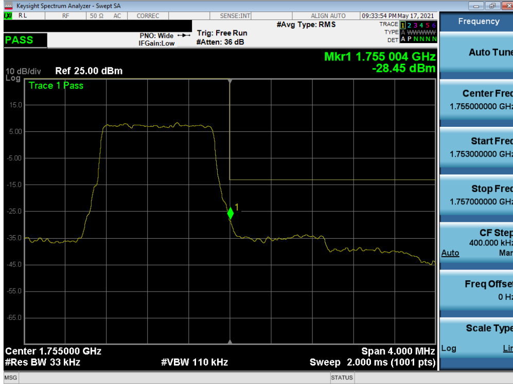
Plot 7-88. Upper Band Edge Plot (LTE Band 4 – 1.4MHz QPSK – Full RB)
