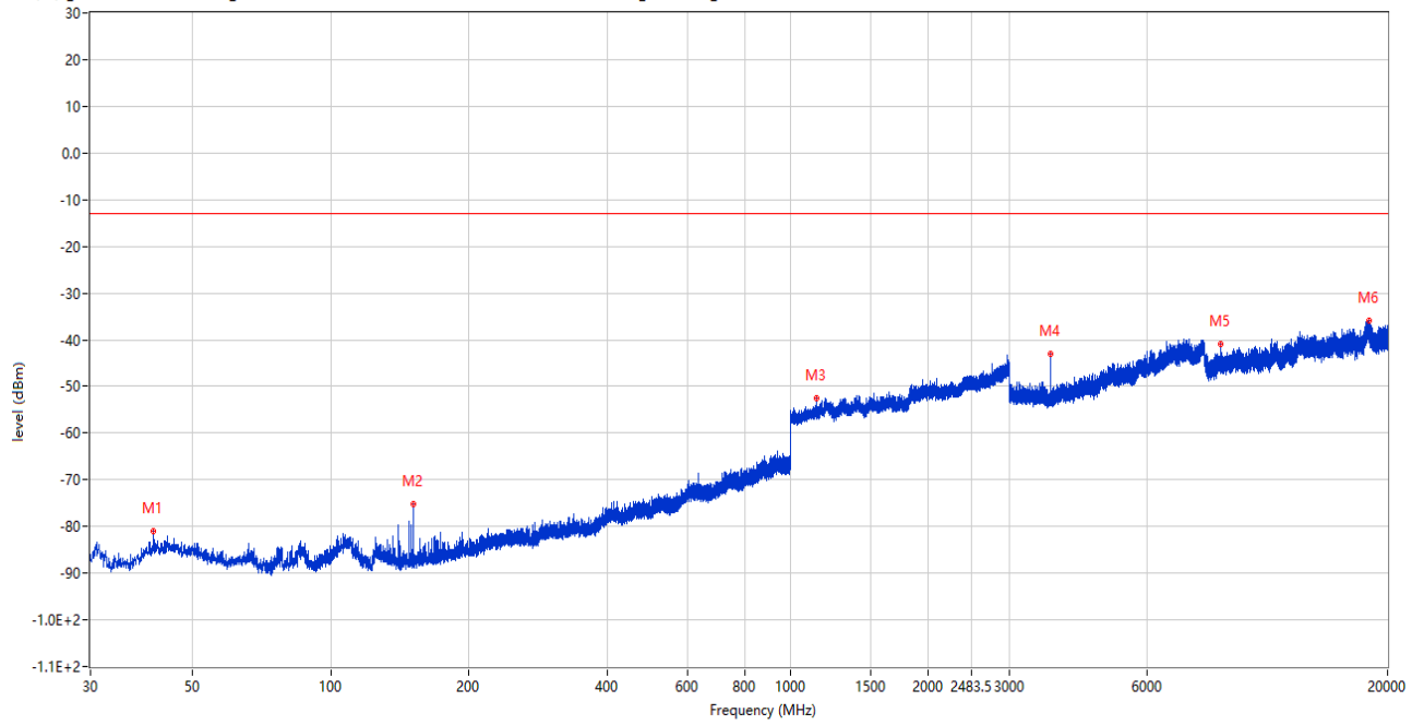
RSE (RF) _FCC PART22&24&27-RSE_GSM 1900 & CDMA BC1 & WCDMA Band 2 & LTE Band 2 & 25_1830-1920_30MHz-20GHz
