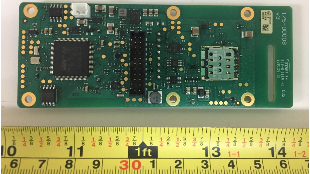
EUT Cover Off View-Bottom
