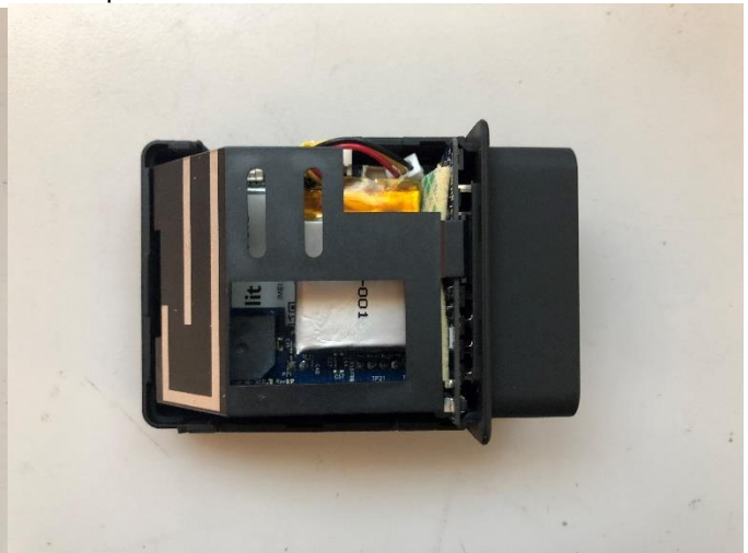
EUT top view without shield
