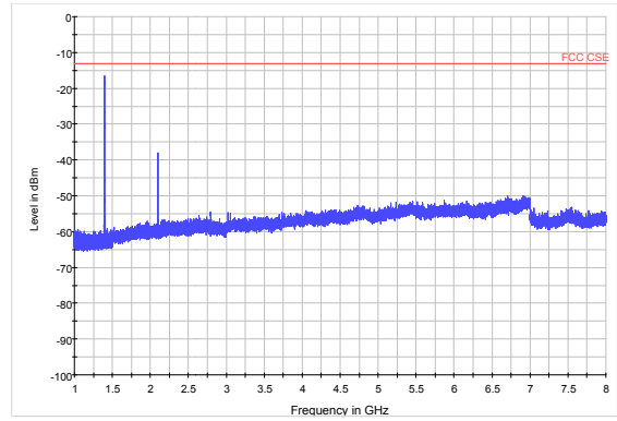
NB-IOT Band 12 CH-Middle 1GHz~8GHz
