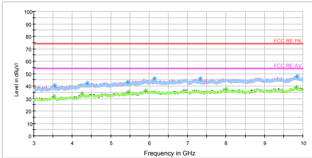
Radiated Emission from 3GHz to 10GHz
