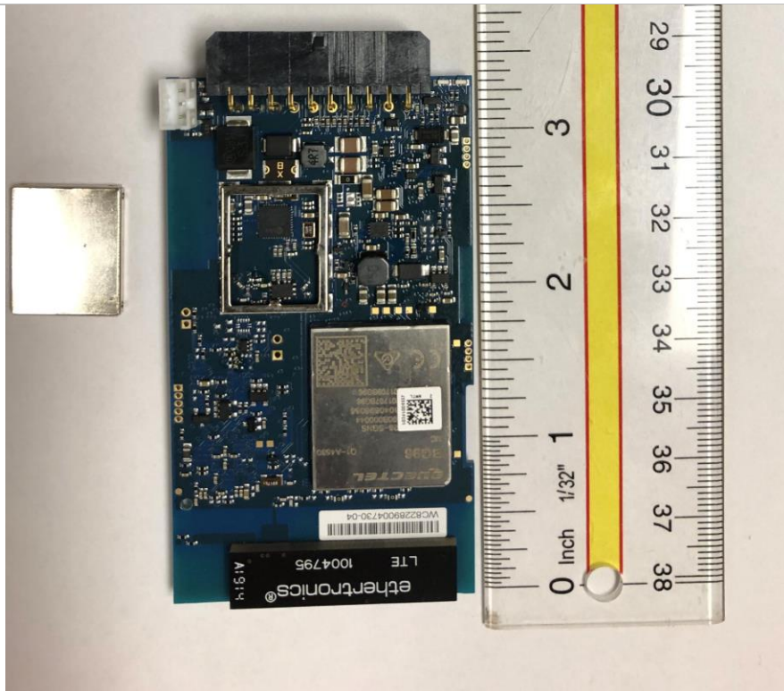
EUT Cover Off View-Top without shielding -2
