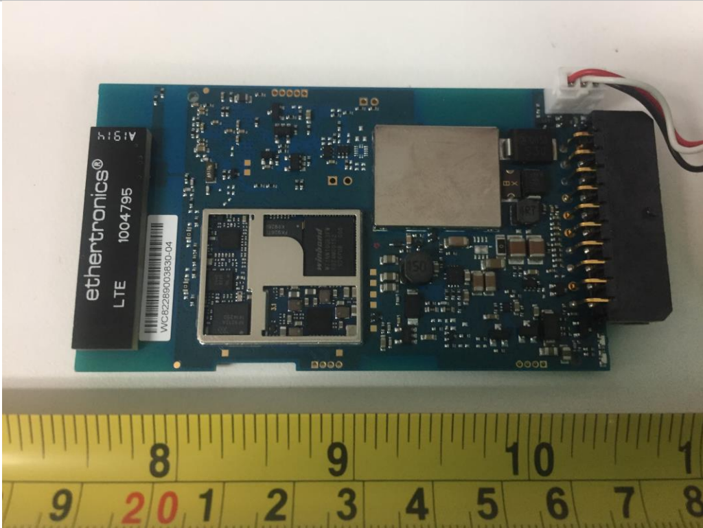
EUT Cover Off View-Top without shielding -1
