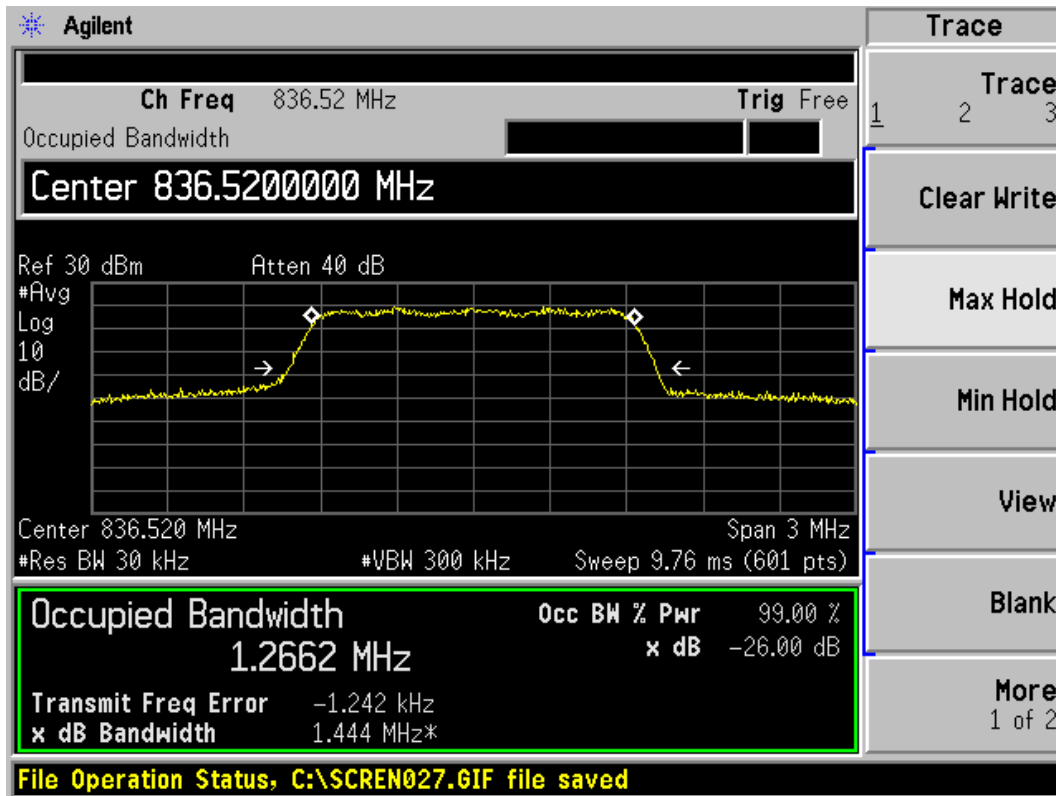
CDMA Cellular RC1 (SO2) CH384 Occupied Bandwidth
