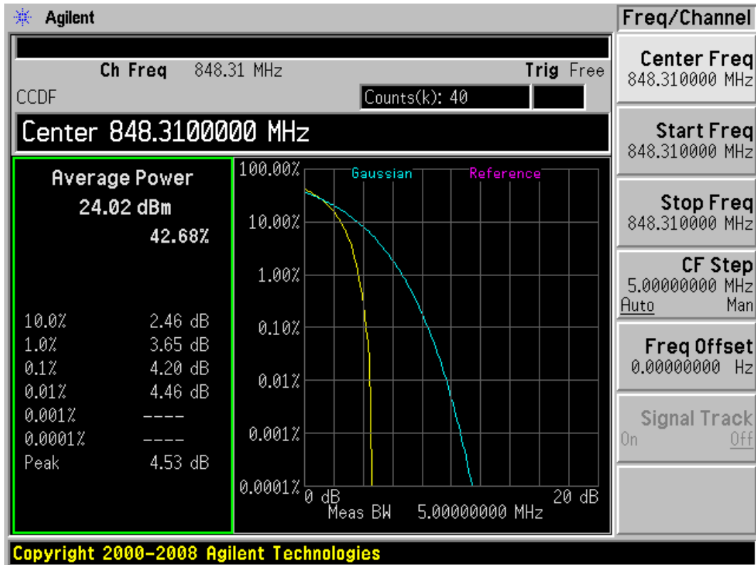
CDMA Cellular RC1 (SO2) CH777
