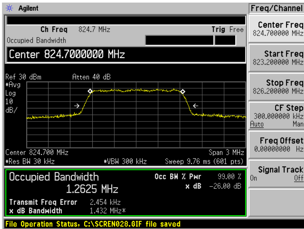
CDMA Cellular RC1 (SO2) CH1013 Occupied Bandwidth
