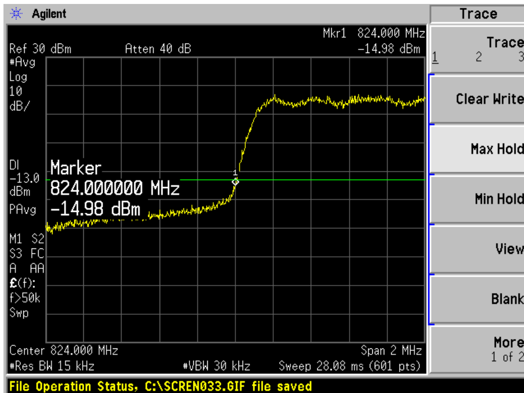
CDMA Cellular RC1 (SO2) 1013 Channel
