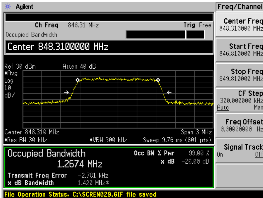
CDMA Cellular RC1 (SO2) CH777 Occupied Bandwidth
