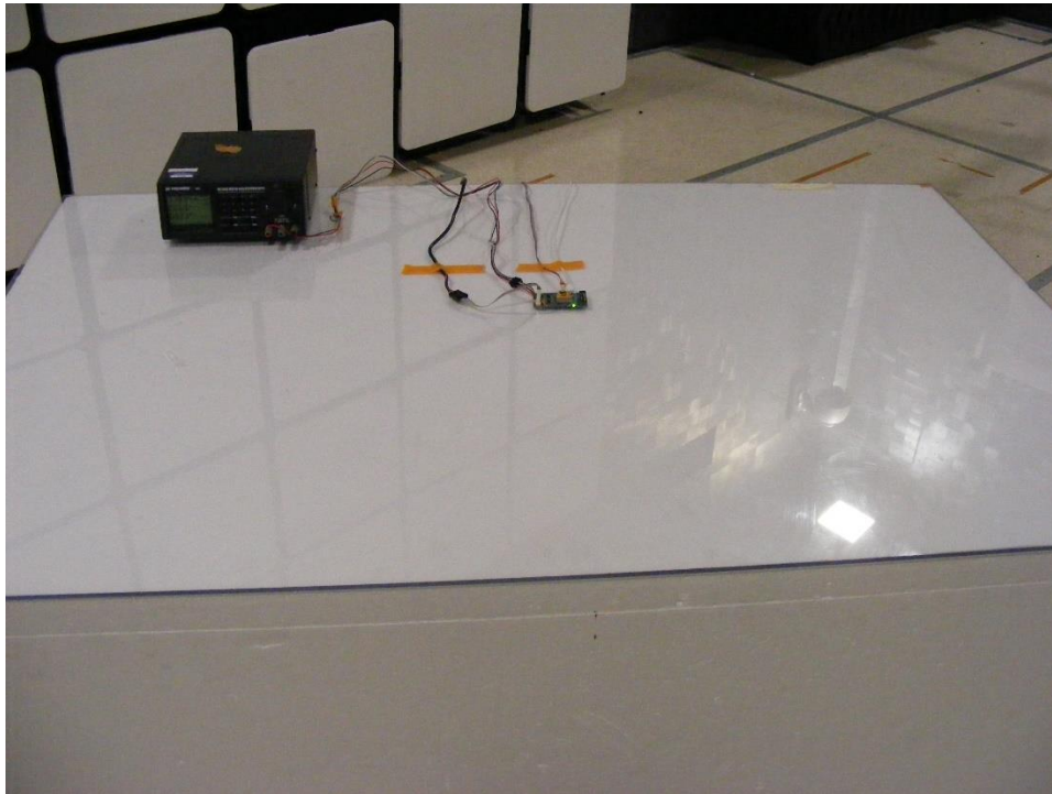
Figure 5a - Radiated emissions Close up view
