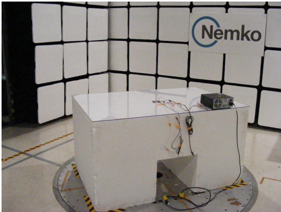
Figure 2 - Radiated emissions below 1 GHz, back view
