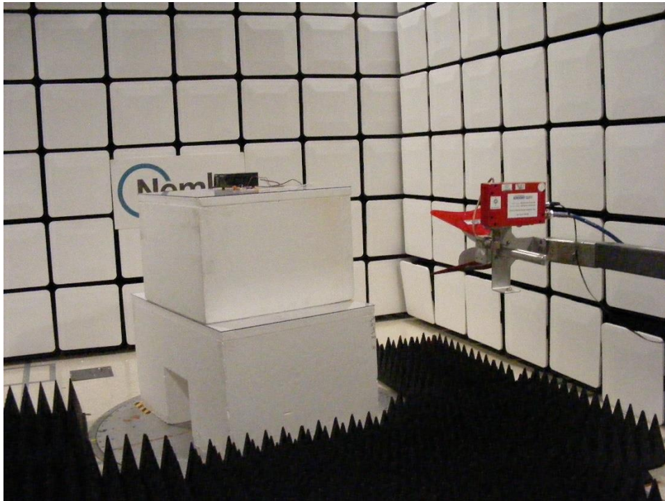
Figure 3 - Radiated emissions above 1 GHz, front view
