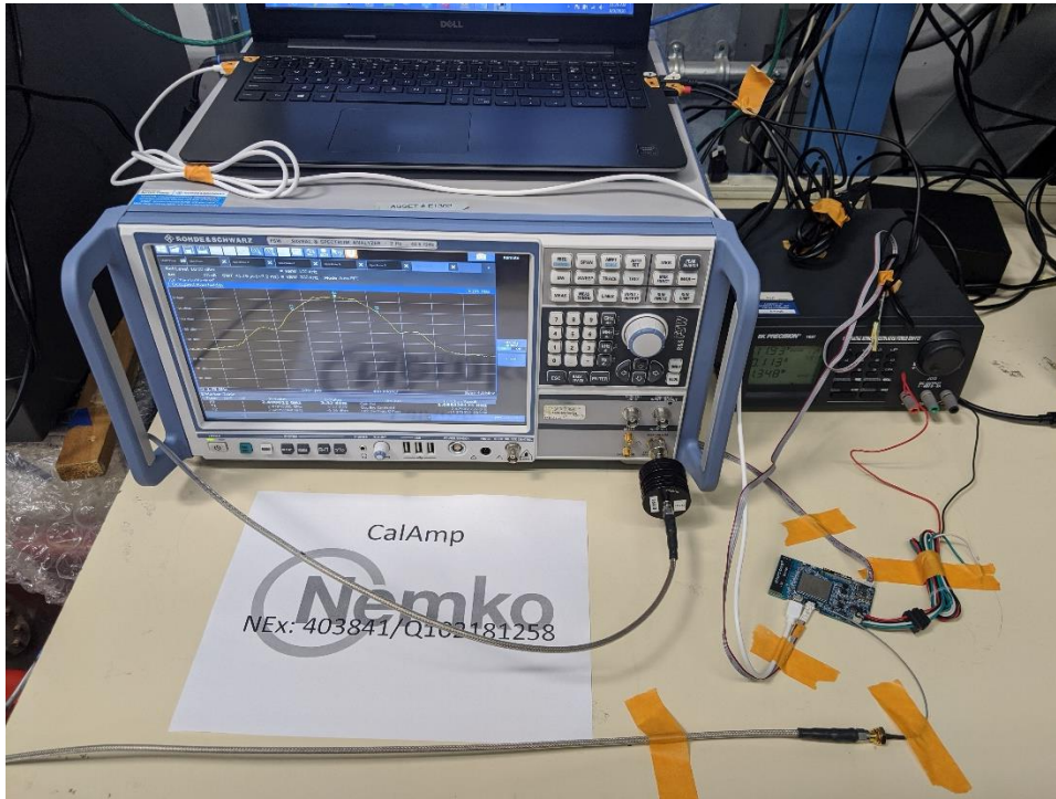
Figure 8 – Conducted antenna port test setup
