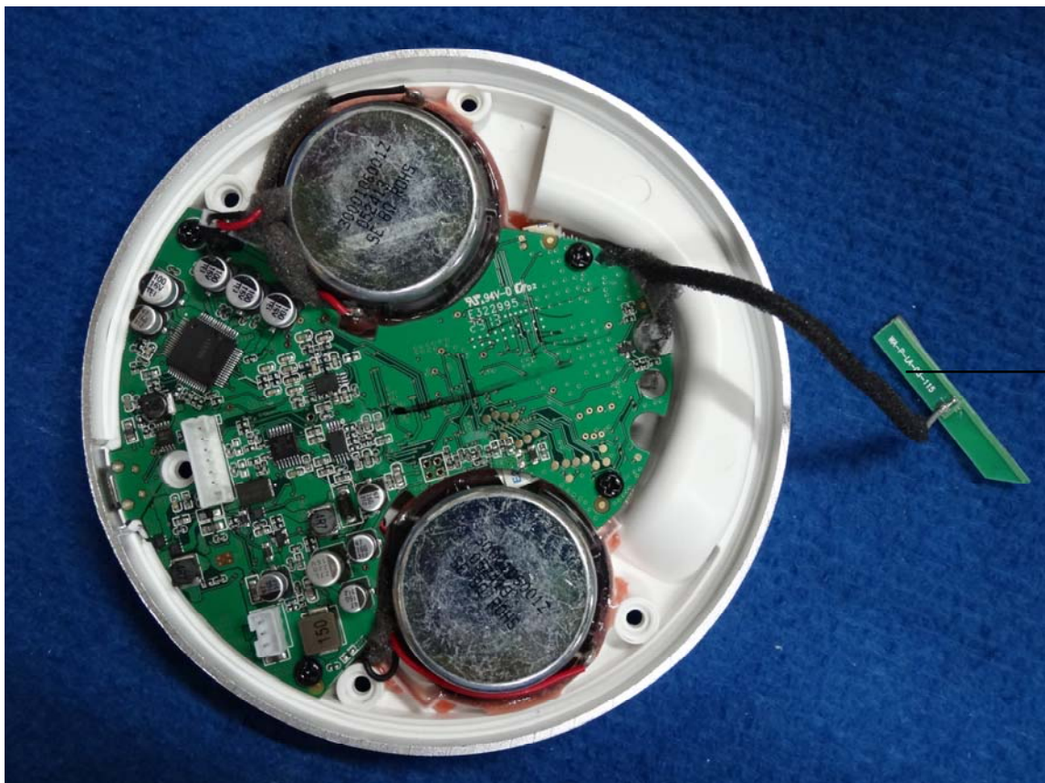
portable unit
