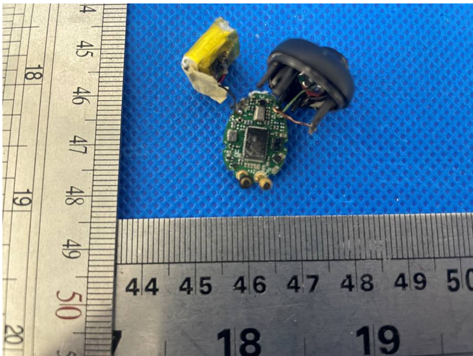
Figure 8 PCB view 1 of R ear bud
