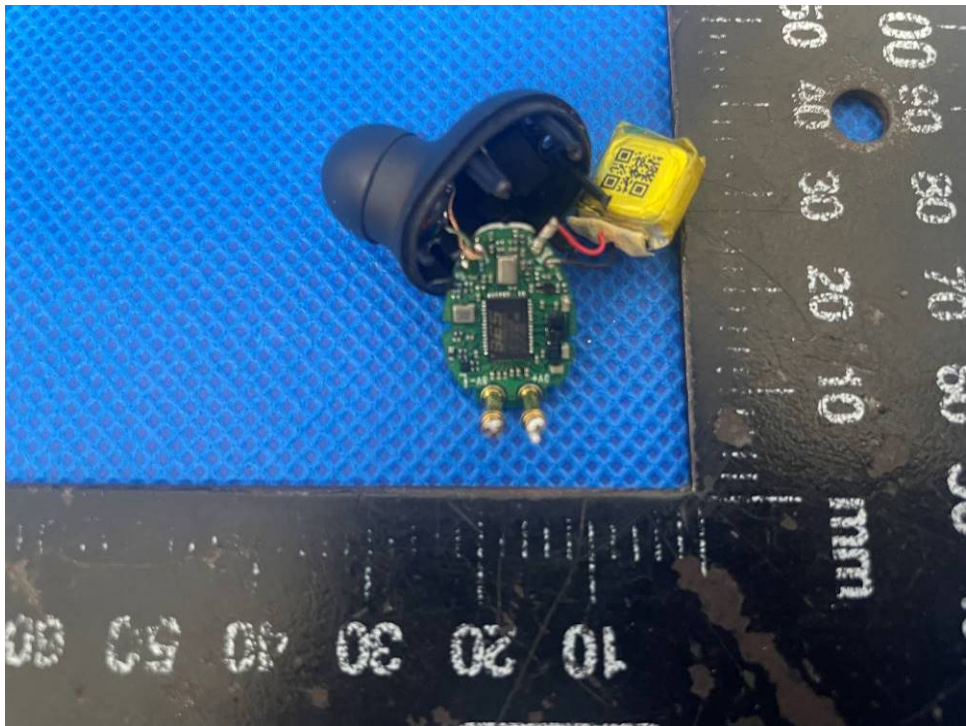
Figure 7 PCB view 2 of L ear bud
