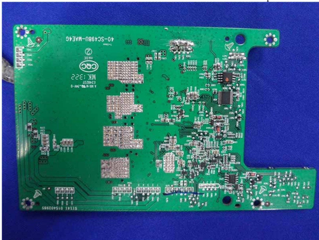
Figure 20 Components Side of the PCB
