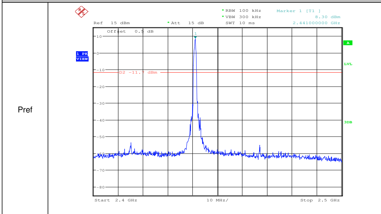
RF Conducted Spurious Emissions_3DH5_2441
