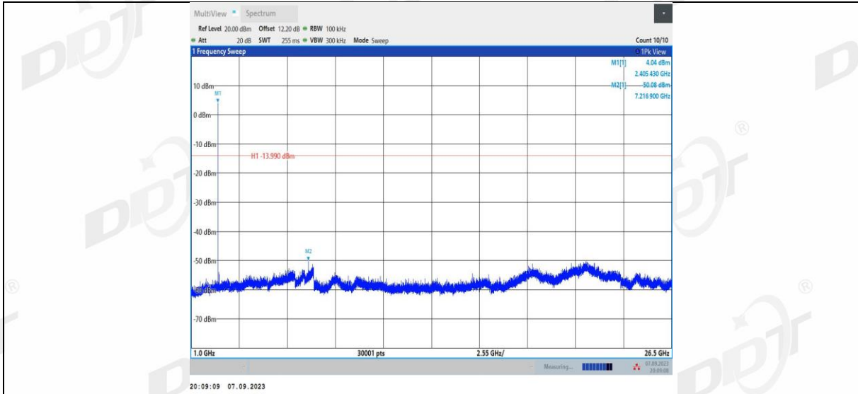
GFSK_2M_Ant1_2442_0~Reference
