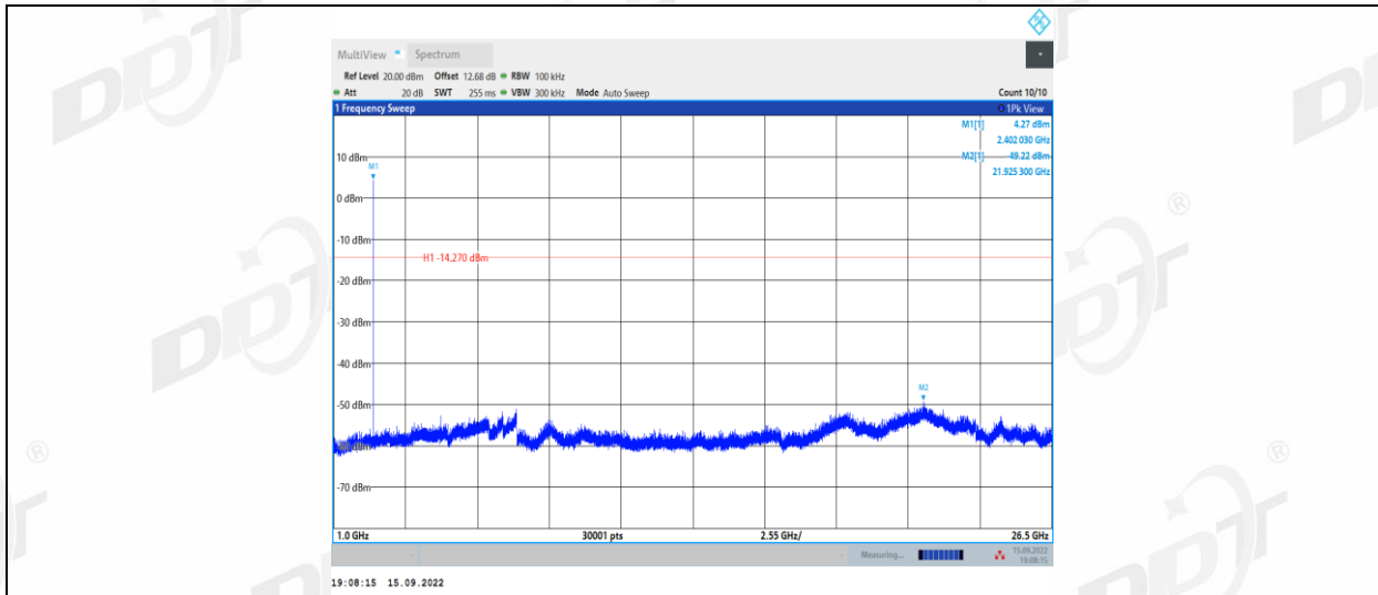
GFSK_2M_Ant1_2440_0-Reference
