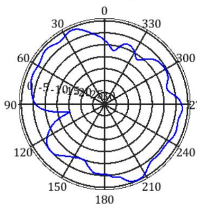
frequency=2400MHz, X-Y Plane
