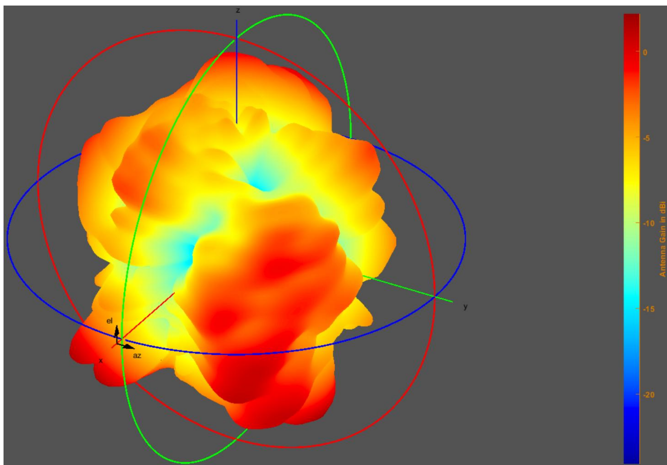
2400MHz_3D
