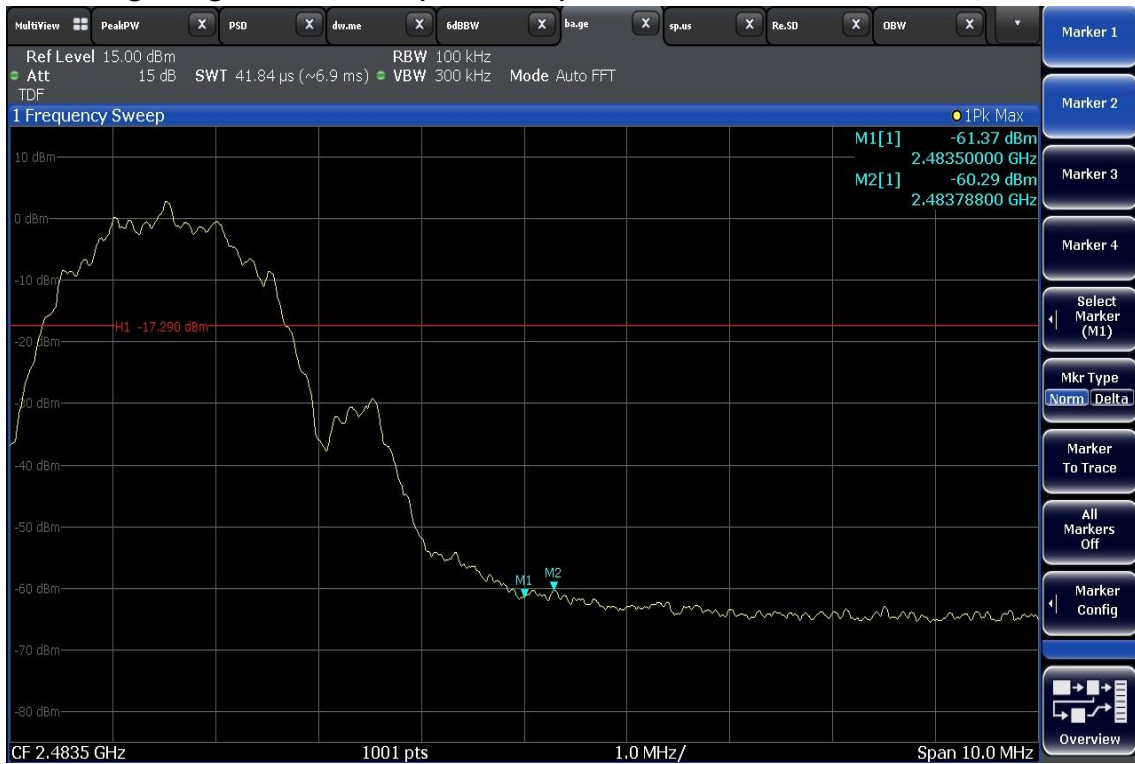
Band Edge, Highest Channel (2480 MHz)
