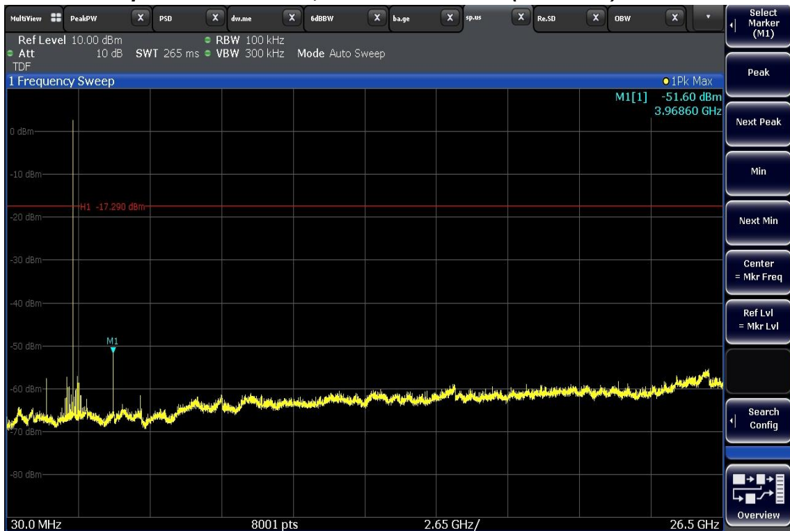
Conducted Spurious Emissions, 30 MHz ~ 26.5 GHz (2480 MHz)
