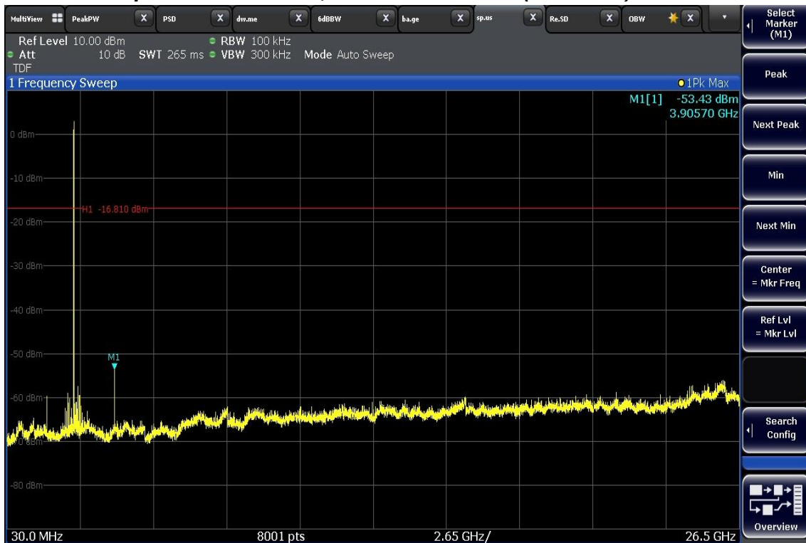
Conducted Spurious Emissions, 30 MHz ~ 26.5 GHz (2442 MHz)
