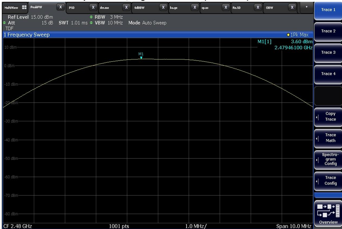
Maximum Peak Output Power, Highest Channel (2480 MHz)
