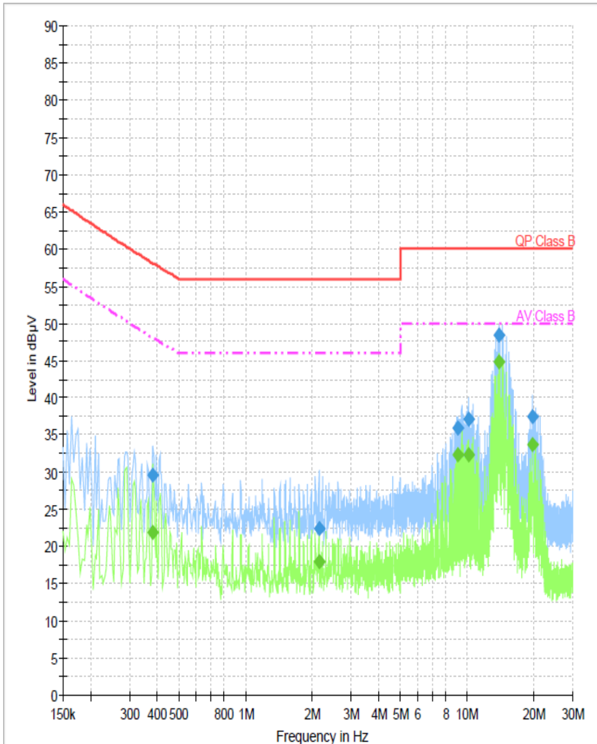
Conducted Emission at the Mains port (Line + Neutral) _2442 MHz
