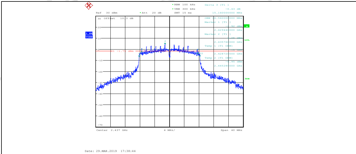
11G_ANT2_2437_6dB Bandwidth
