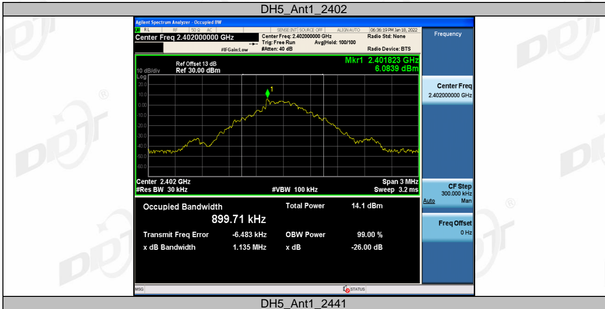
99% Bandwidth
