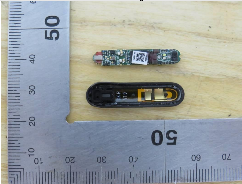
Internal View of EUT- Right Earbud-2
