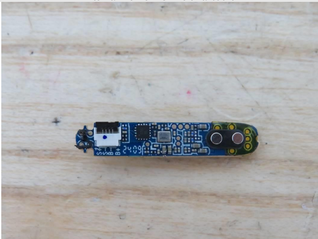
Internal View of EUT-Left Earbud-6
