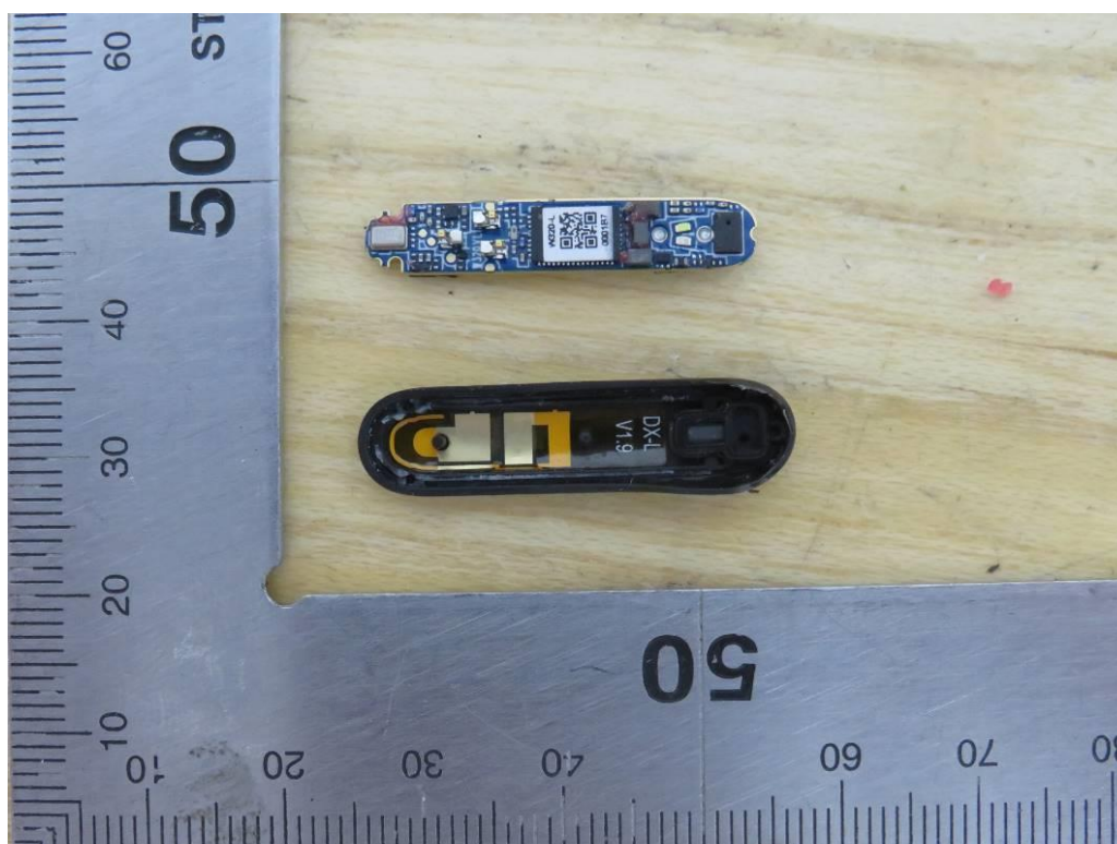
Internal View of EUT-Left Earbud-2
