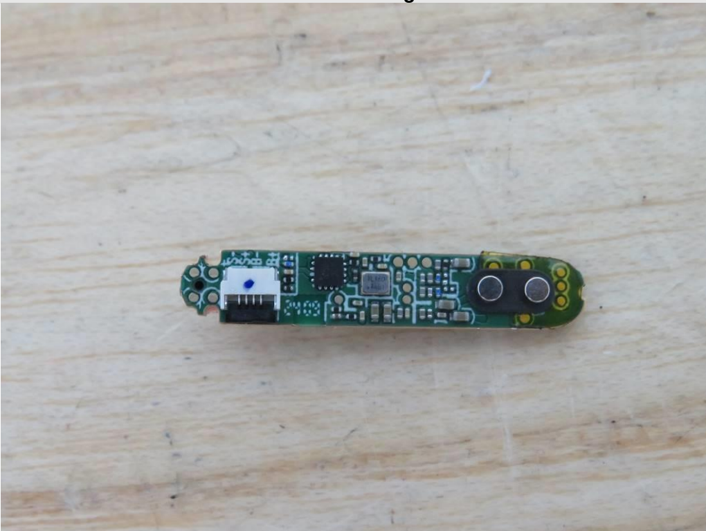
Internal View of EUT-Right Earbud-5
