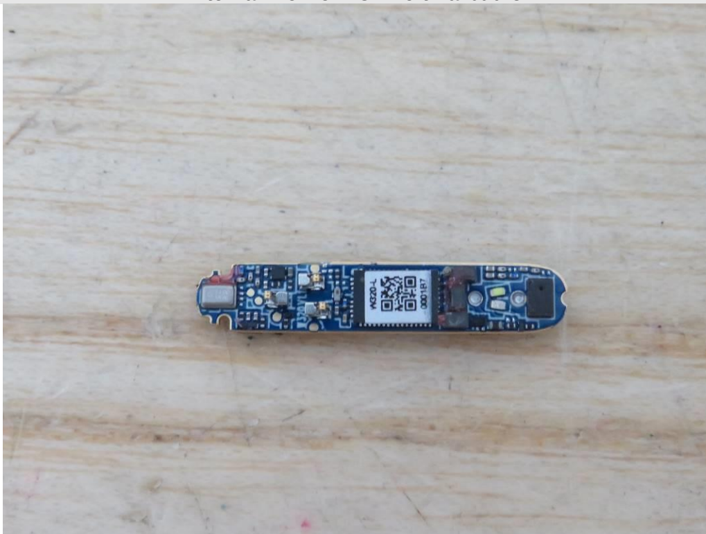
Internal View of EUT-Left Earbud-5
