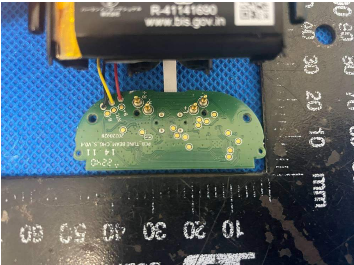
Figure 9 PCB view 2(Charging case)
