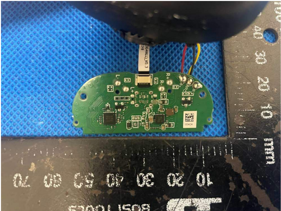
Figure 8 PCB view 1(Charging case)
