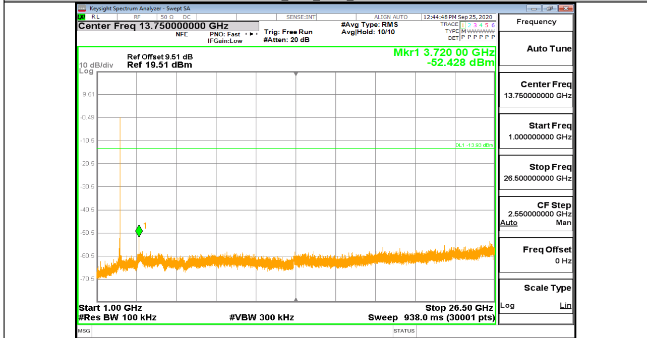
3DH5_Ant1_2480_1000~26500
