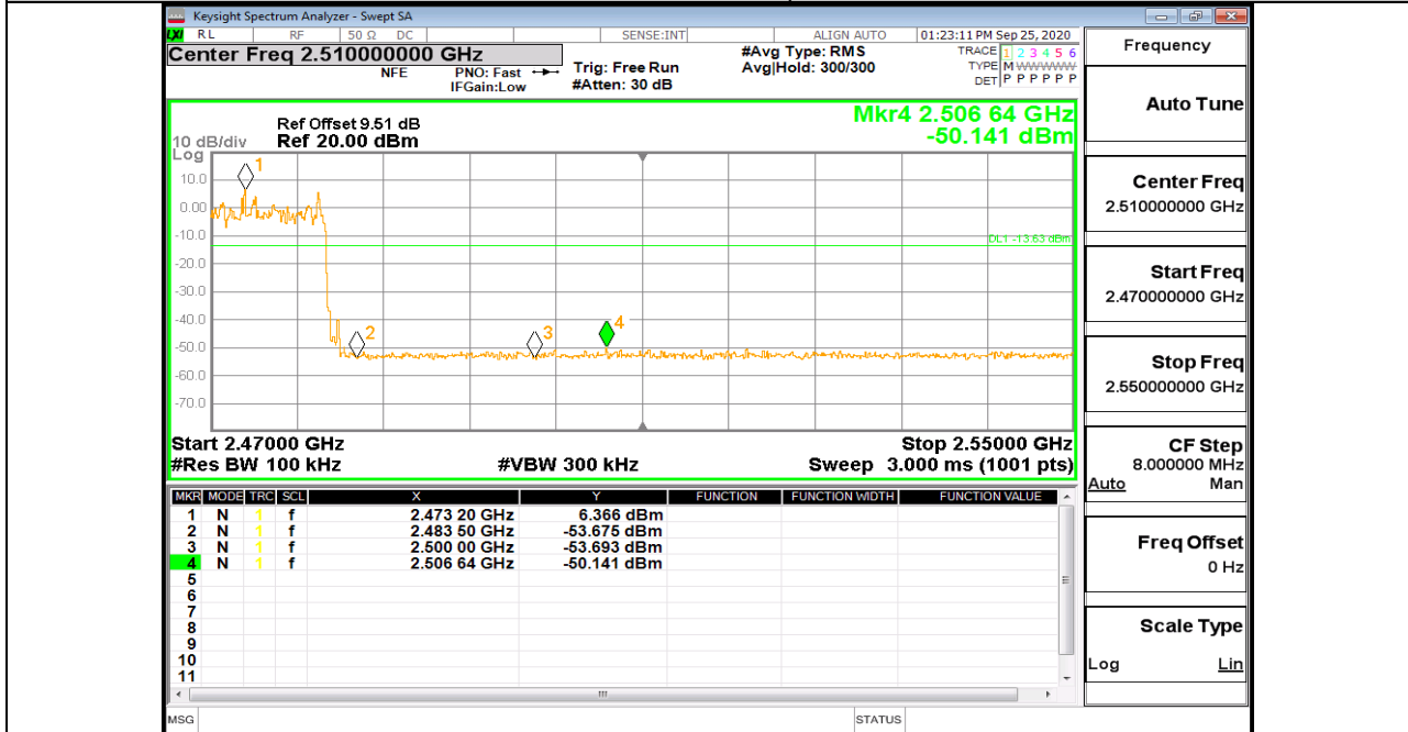
3DH5_Ant1_High_Hop_2480
