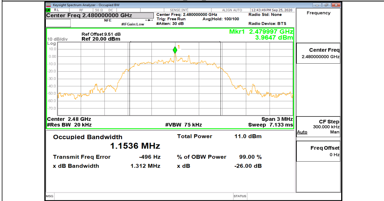
3DH5_Ant1_2480
