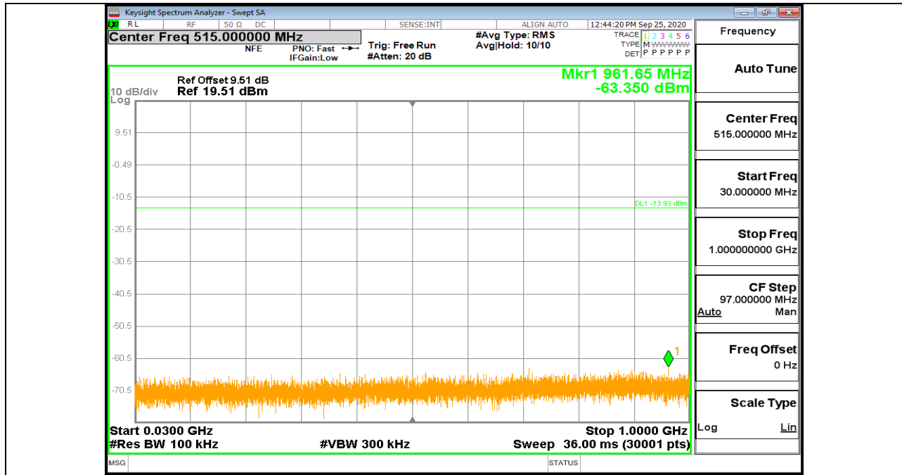
3DH5_Ant1_2480_30~1000
