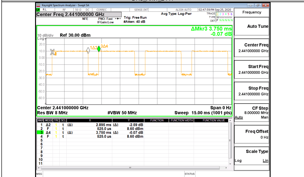
3DH5_Ant1_2441
