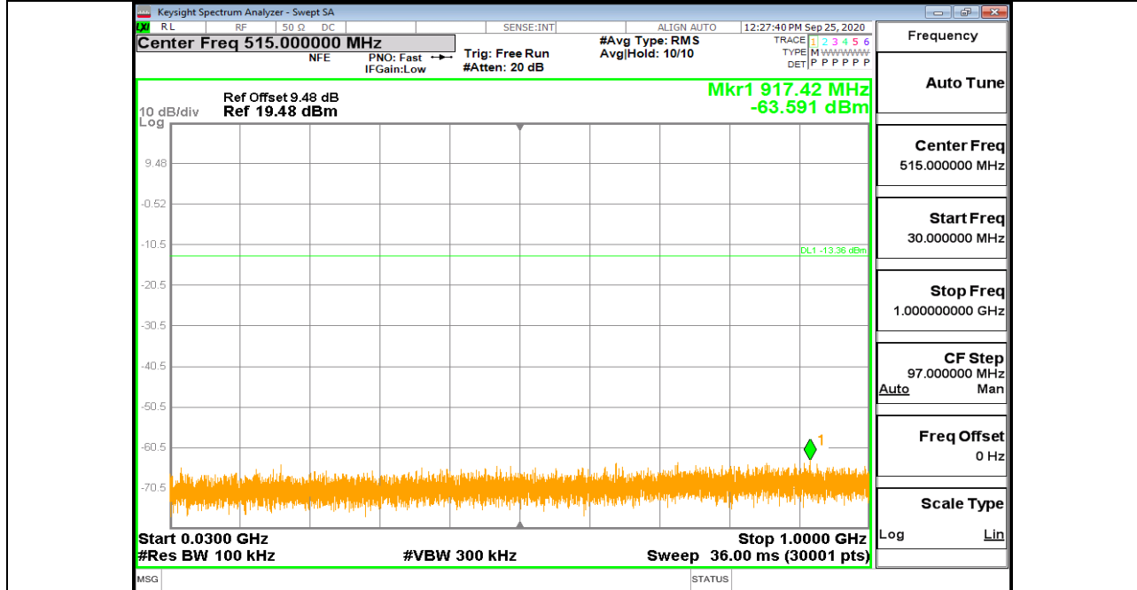
DH5_Ant1_2402_30-1000
