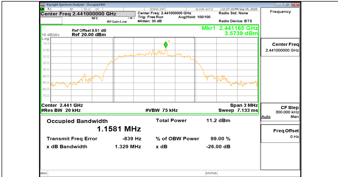
3DH5_Ant1_2441
