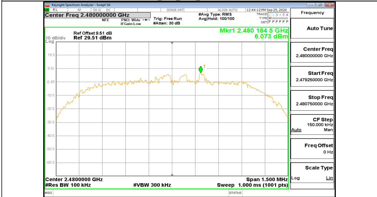
3DH5_Ant1_2480_0~Reference
