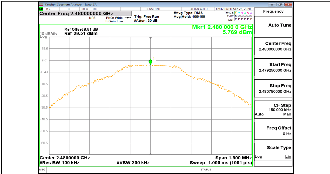
DH5_Ant1_2480_0~Reference
