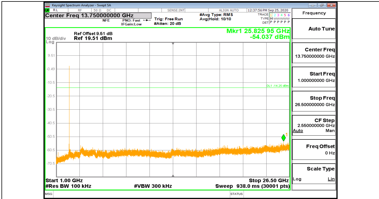
3DH5_Ant1_2441_1000~26500
