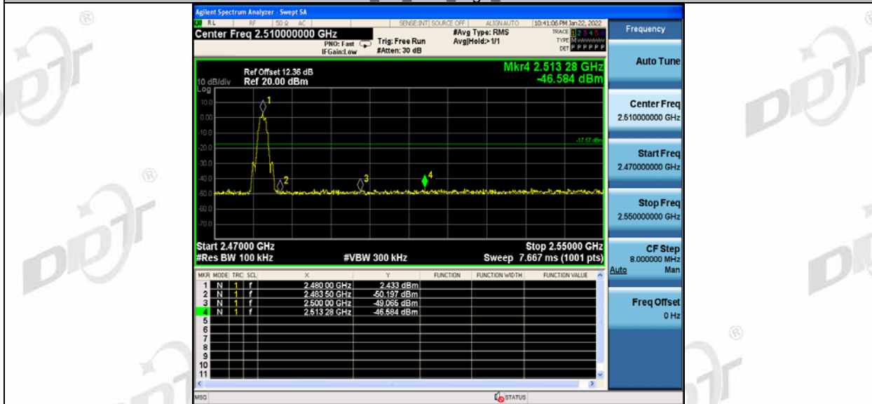
BLE_2M_Ant1_High_2480
