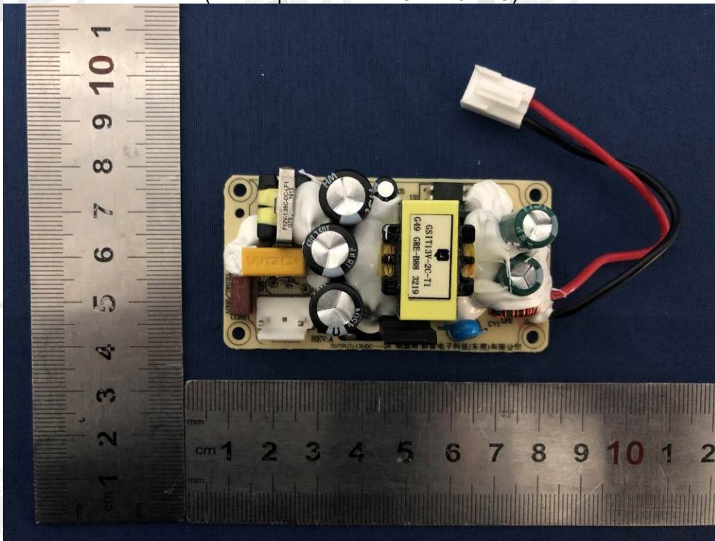
(Built-in power board: GSIT13V-2C)
