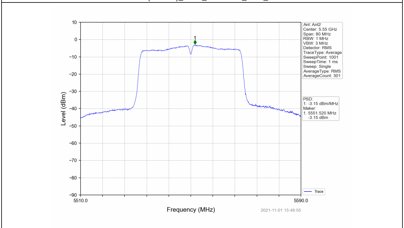
802.11ac(VHT40)_MCH_5550MHz_Ant2_NTNV
