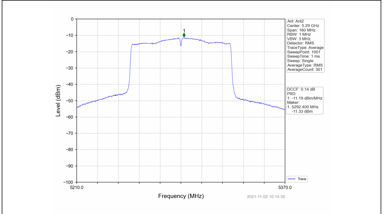
802.11ac(VHT80)_MCH_5290MHz_MIMO_NTNV
