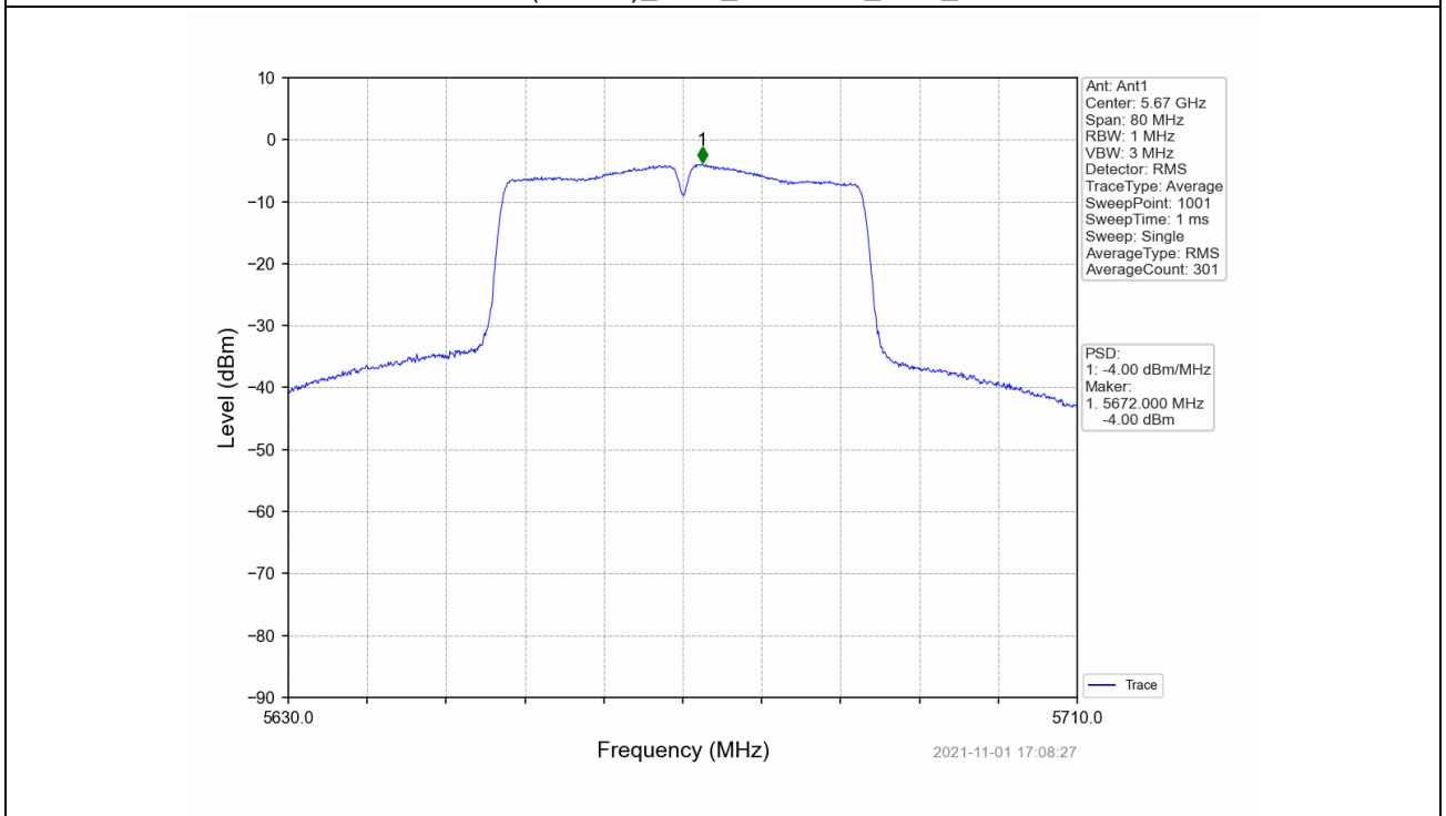
802.11ac(VHT40)_HCH_5670MHz_Ant1_NTNV
