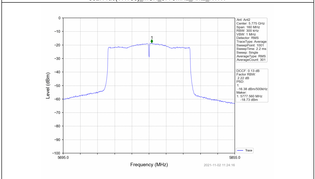
802.11ac(VHT80)_MCH_5775MHz_Ant2_NTNV
