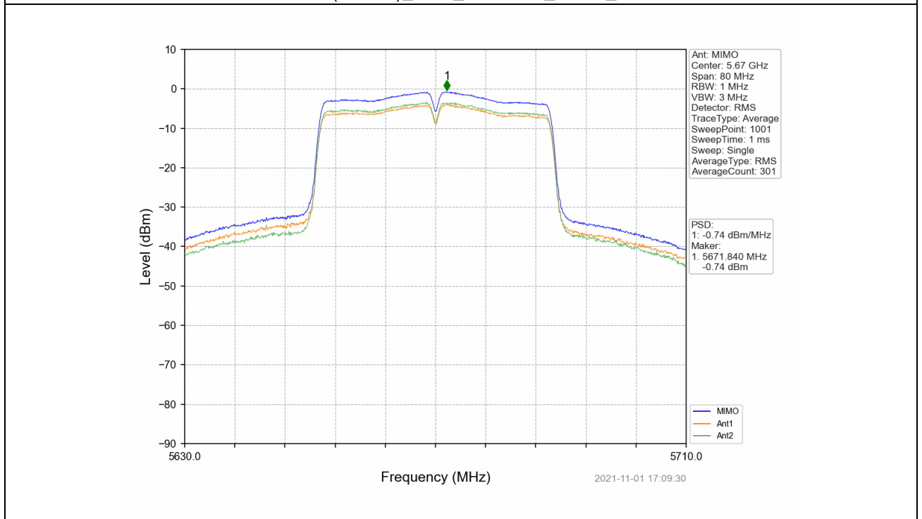
802.11ac(VHT40)_HCH_5670MHz_MIMO_NTNV
