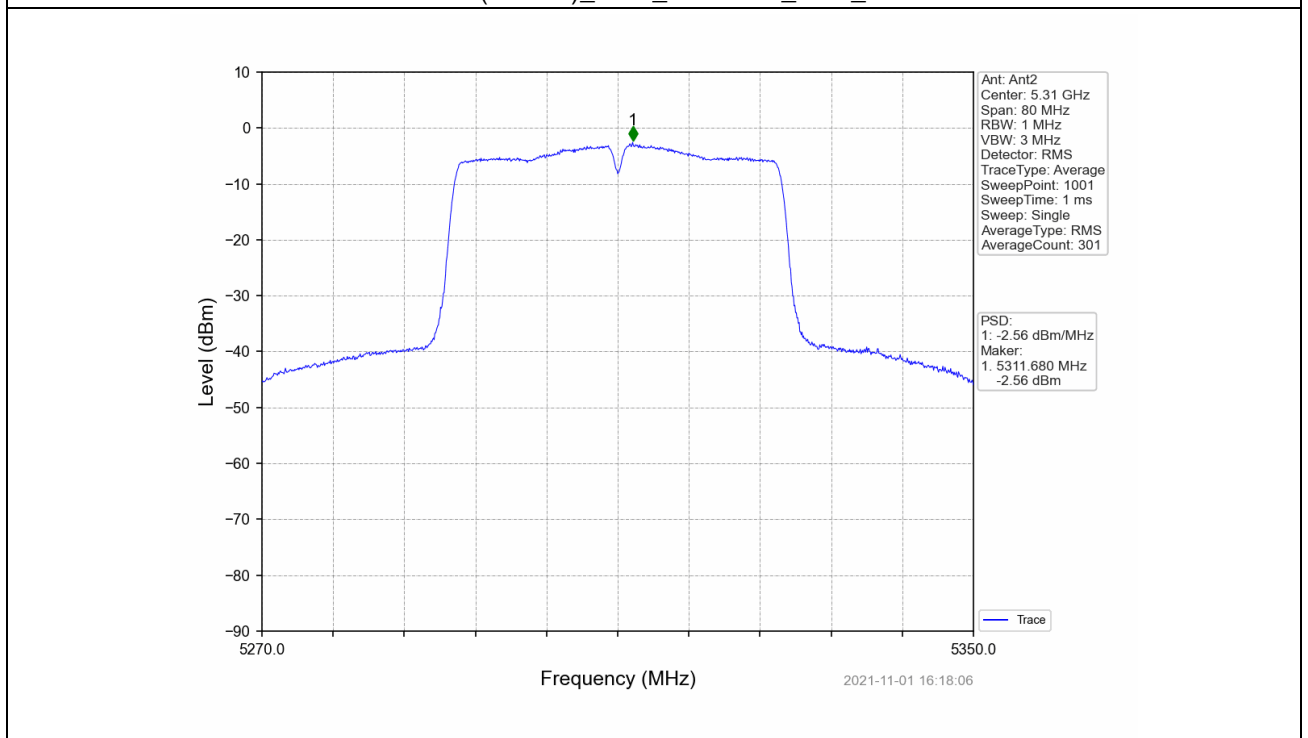
802.11ac(VHT40)_HCH_5310MHz_Ant2_NTNV
