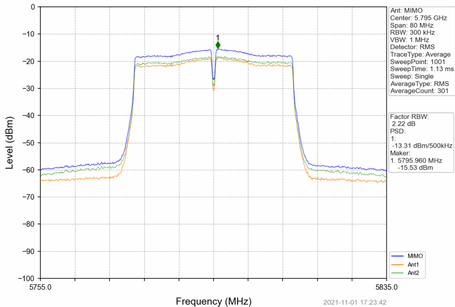
802.11ac(VHT40)_HCH_5795MHz_MIMO_NTNV
