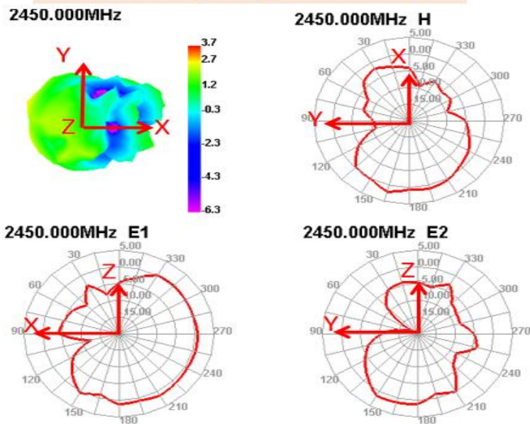
WIFI-1天线_2.4G_方向图2D/3D
