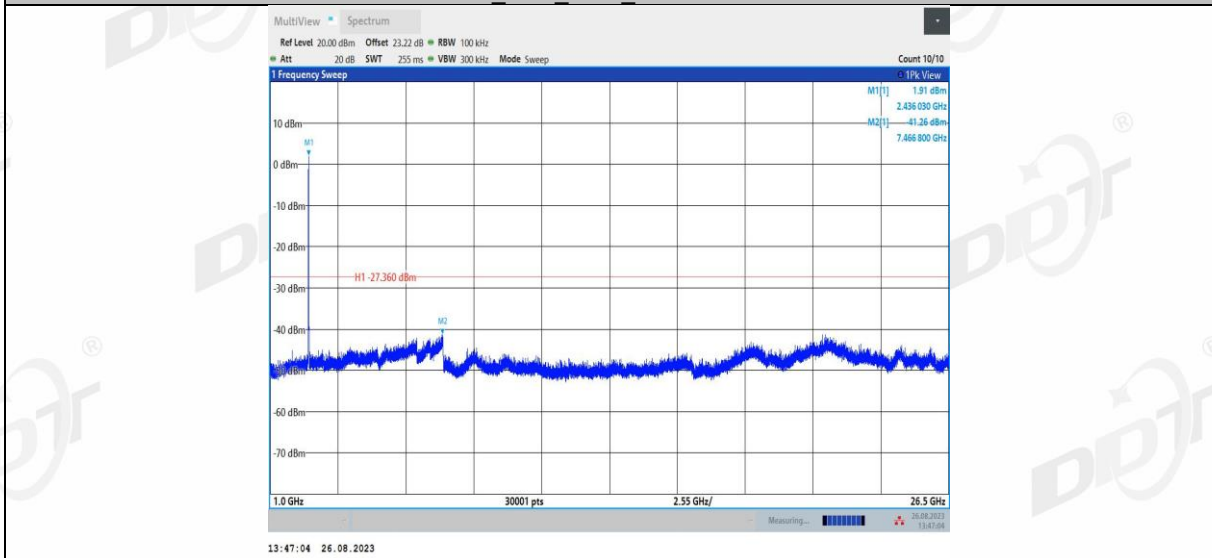
11G_Ant2_2437_0~Reference
