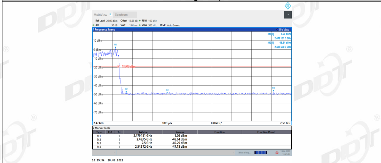
3DH5_Ant1_High_Hop_2480
