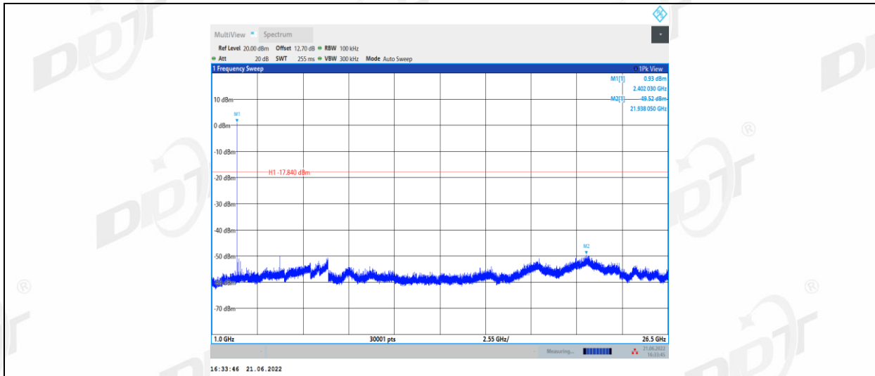
3DH5_Ant1_2441_0~Reference
