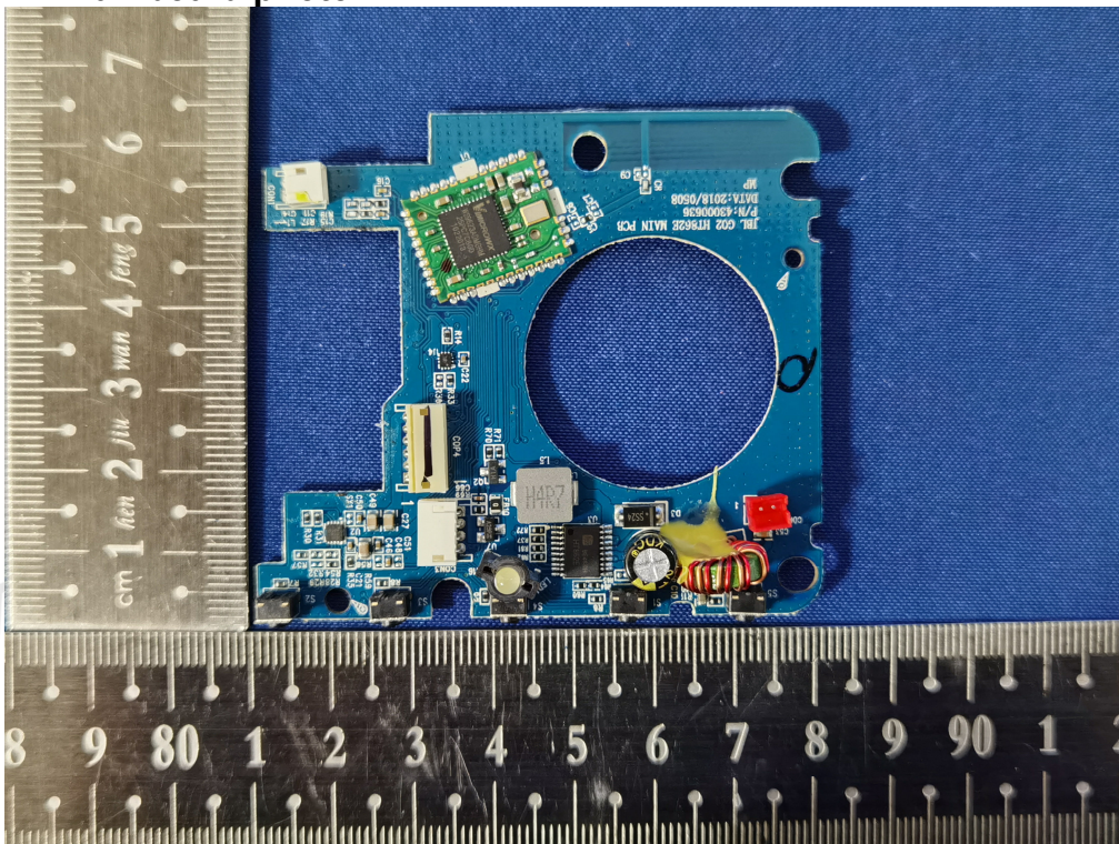
New PCB mainboard photo:
