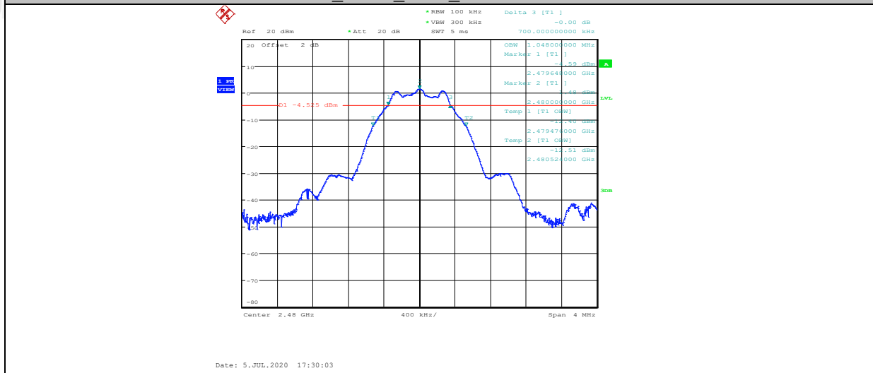
BLE_ANT1_2480_6dB bandwidth
