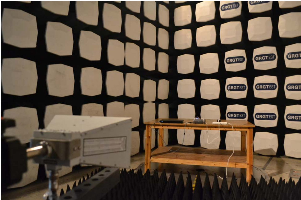
RSE (Above 1GHz)
