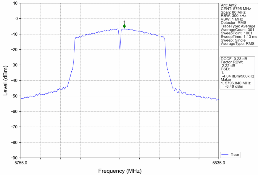
802.11ac(VHT40)_HCH_5795MHz_MIMO_NTNV
