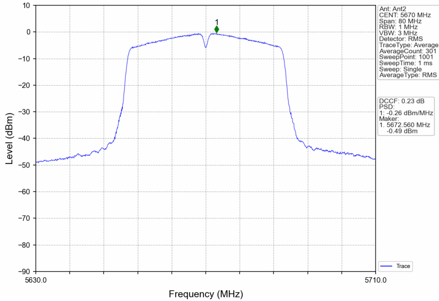
802.11ac(VHT40)_HCH_5670MHz_MIMO_NTNV
