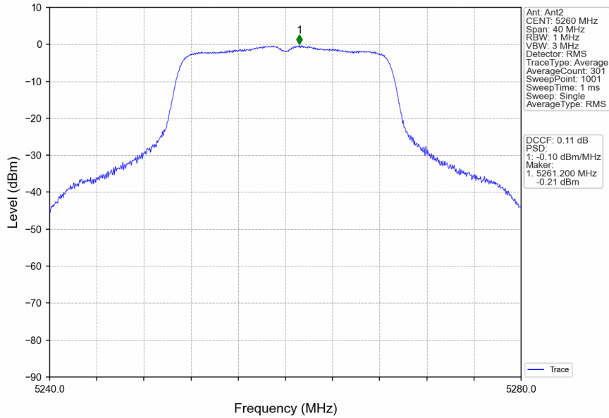
802.11ac(VHT20)_LCH_5260MHz_MIMO_NTNV
