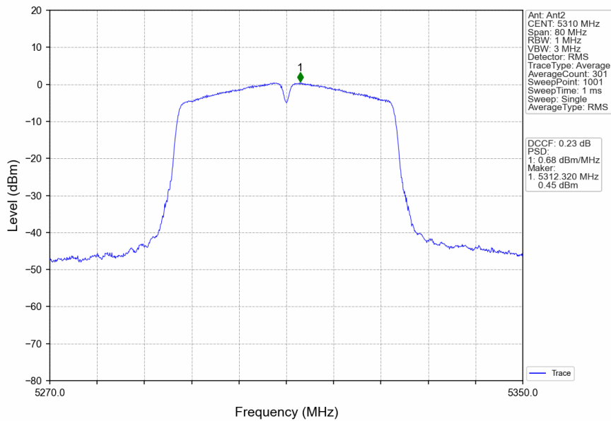
802.11ac(VHT40)_HCH_5310MHz_Ant2_NTNV
