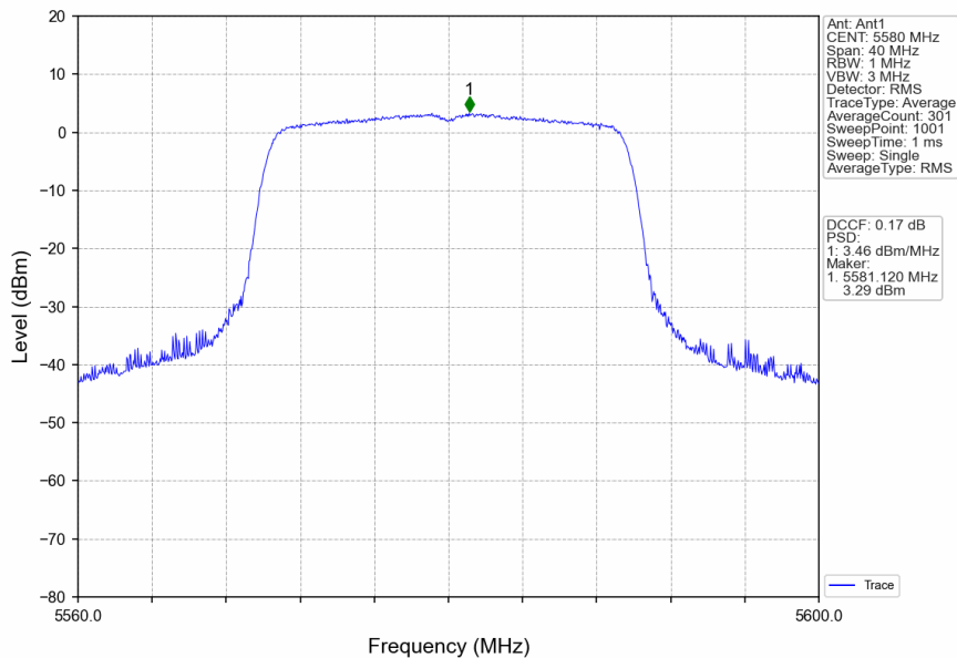
802.11ax(HEW20)_MCH_5580MHz_RU242_Left_Ant1_NTNV
