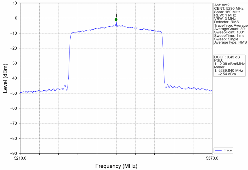
802.11ac(VHT80)_MCH_5290MHz_MIMO_NTNV
