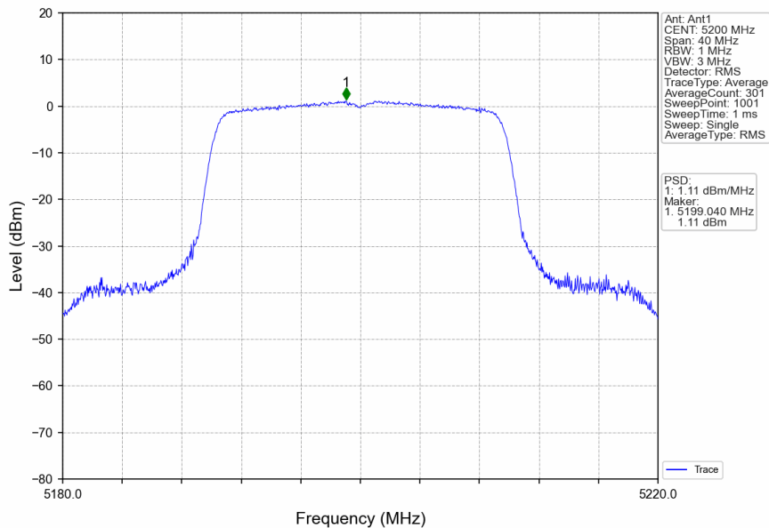
802.11ax(HEW20)_MCH_5200MHz_RU242_Left_Ant1_NTNV
