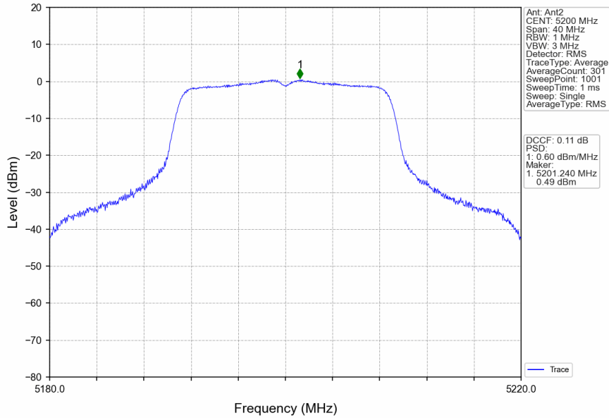
802.11ac(VHT20)_MCH_5200MHz_MIMO_NTNV
