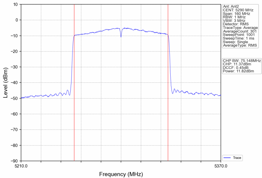
802.11ac(VHT80)_MCH_5290MHz_Ant2_NTNV
