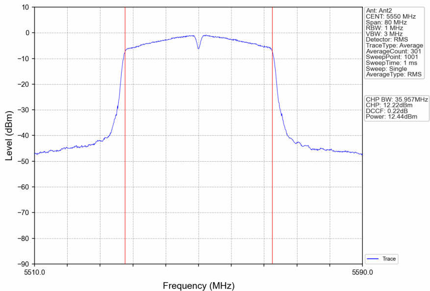
802.11ac(VHT40)_MCH_5550MHz_Ant2_NTNV
