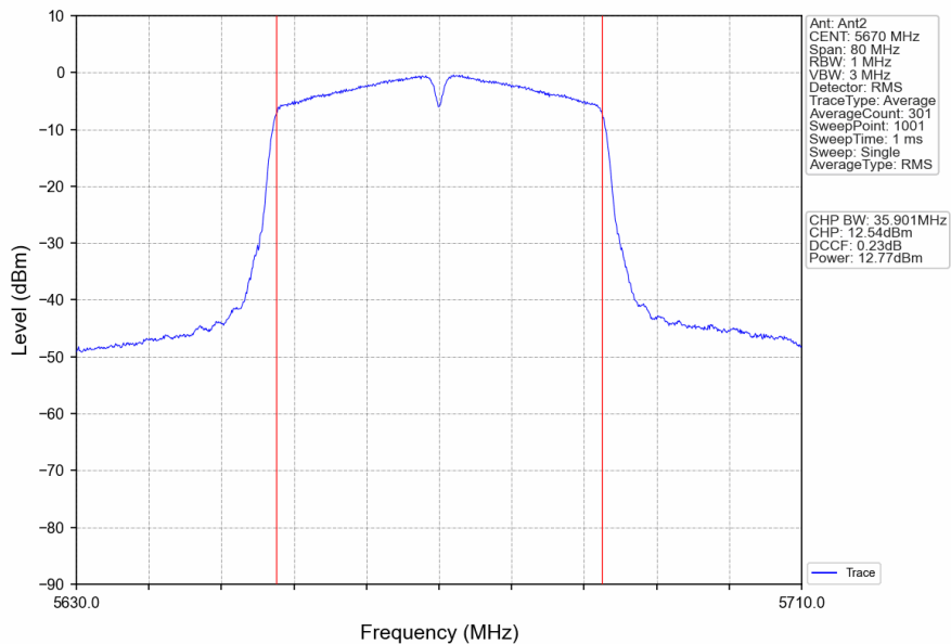
802.11ac(VHT40)_HCH_5670MHz_Ant2_NTNV
