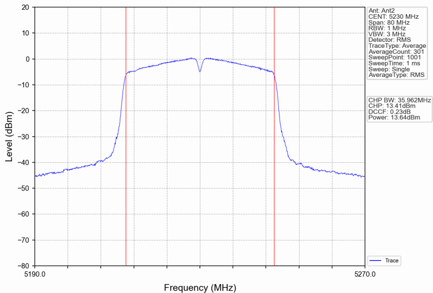
802.11ac(VHT40)_HCH_5230MHz_Ant2_NTNV
