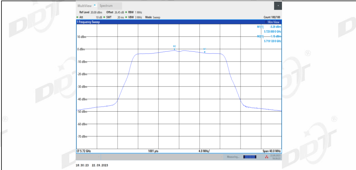
11AC20MIMO Ant2 5720 UNII-2C
