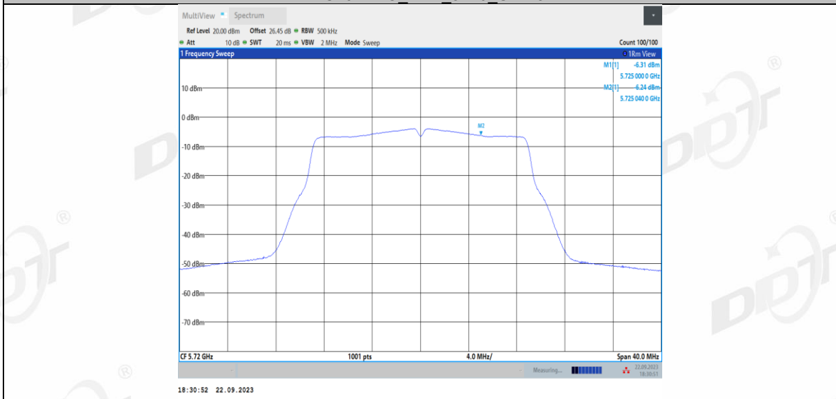
11AC20MIMO Ant2 5720 UNII-3
