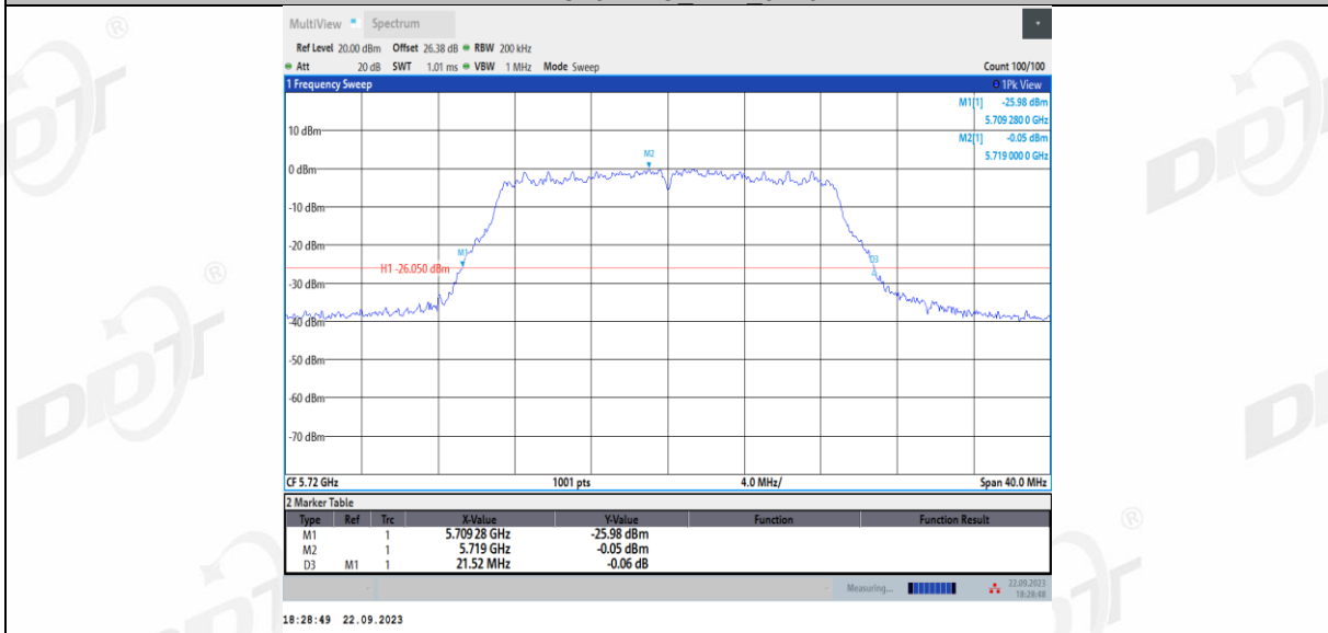
11AC20MIMO Ant2_5720
