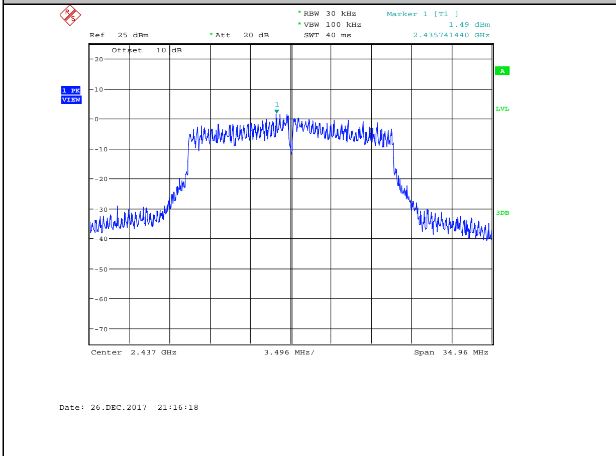
Maximum Peak power spectral density_11N20SISO_2437_Ant2
