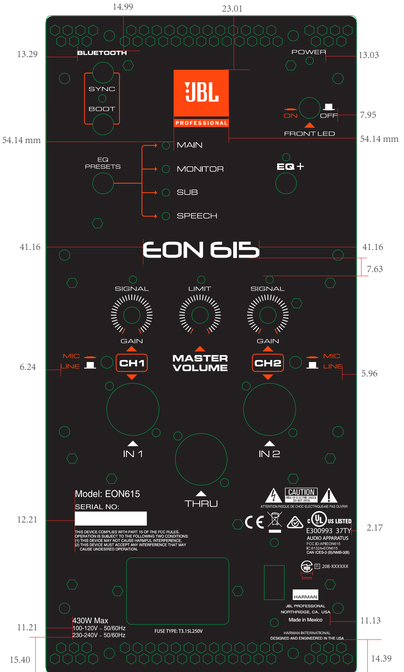
Silkscreen color: White and Pantone 172C T130083400100 V2 ART EON615
