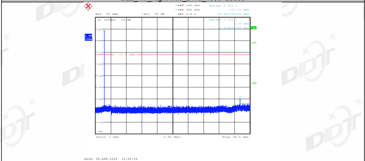
BLE_1M_Left side_2440_0~Reference
