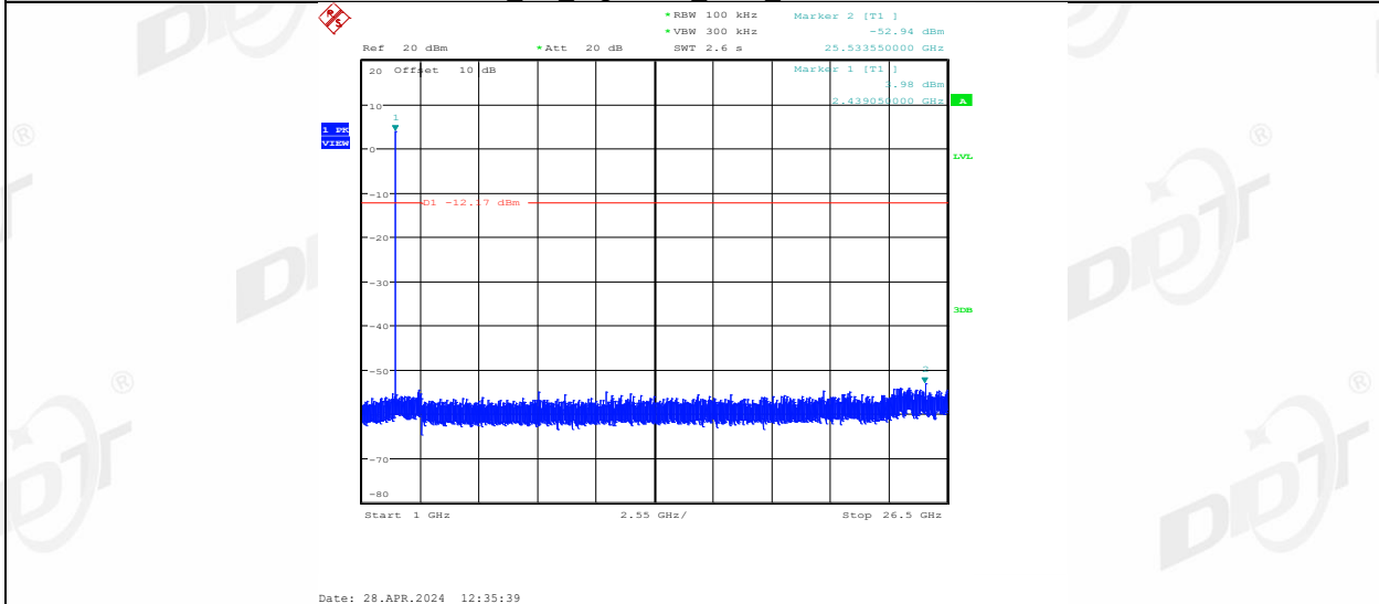
BLE_2M_Left side_2440_0~Reference
