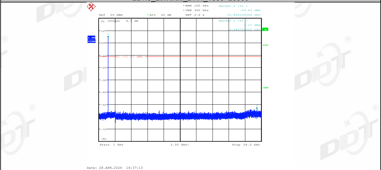
2DH5_Right side_2480_0~Reference
