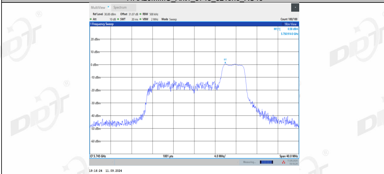
11AX20MIMO Ant1_5745_106Tone_RU53
