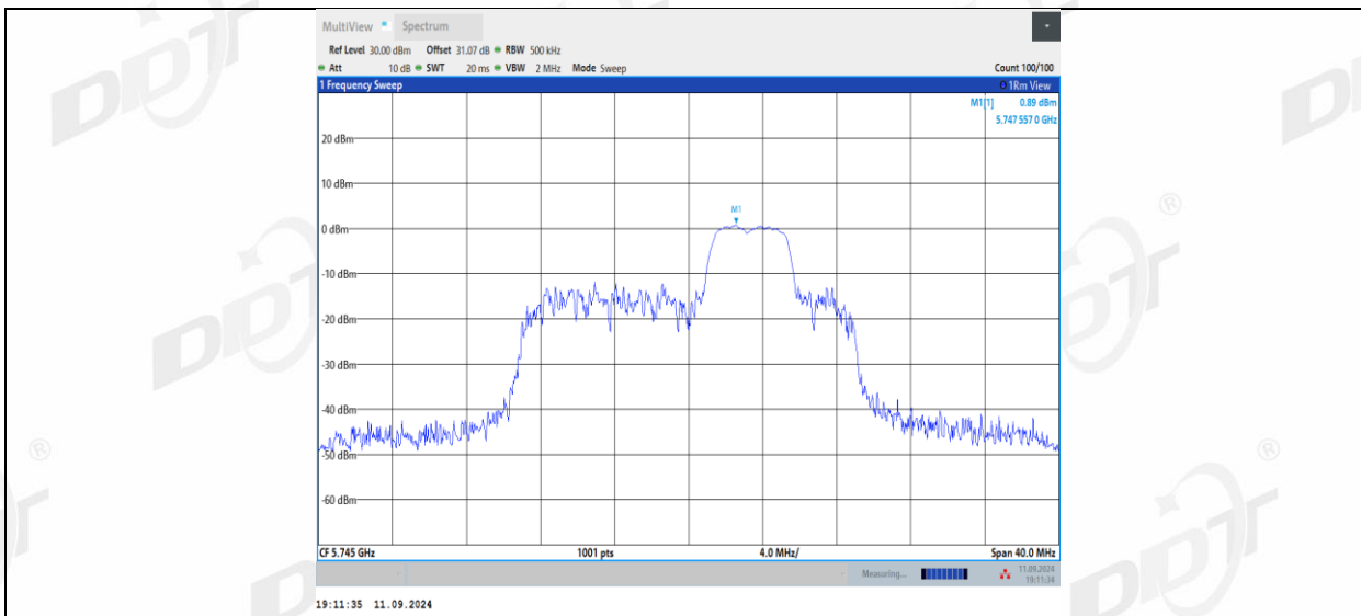
11AX20MIMO Ant1_5745_52Tone_RU40
