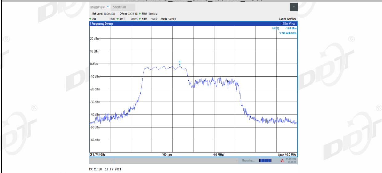
11AX20MIMO Ant1_5745_106Tone_RU54
