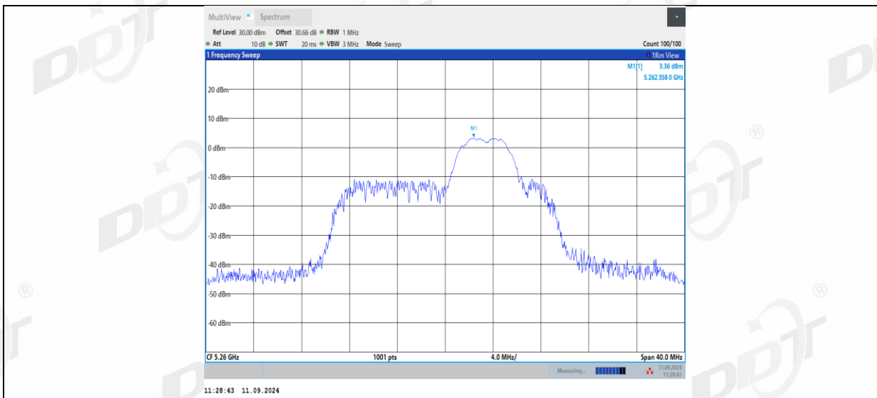
11AX20MIMO Ant1_5260_52Tone_RU40
