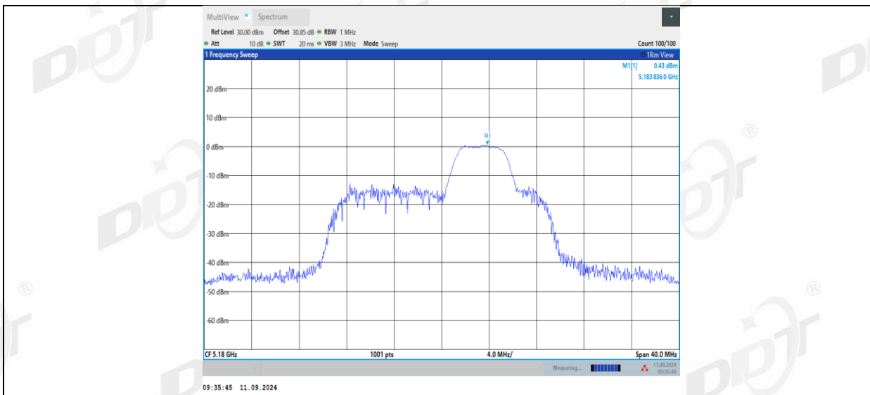
11AX20MIMO Ant1_5180_52Tone_RU40
