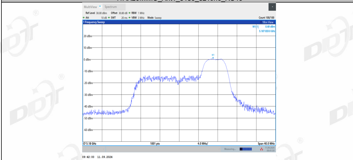
11AX20MIMO Ant1_5180_106Tone_RU53
