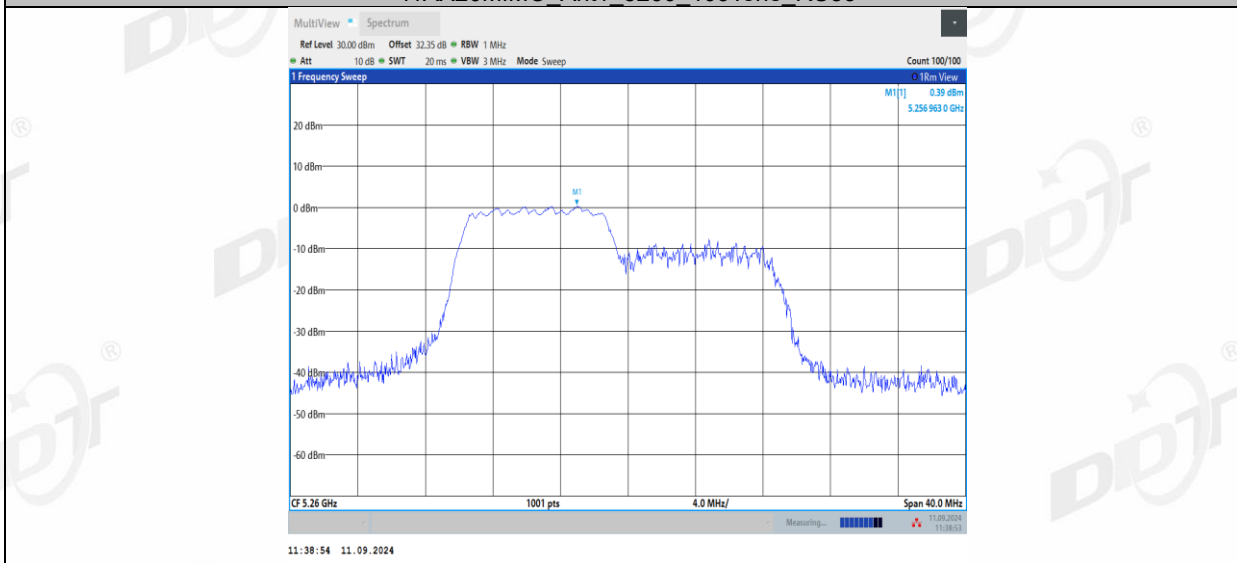
11AX20MIMO Ant1_5260_106Tone_RU54
