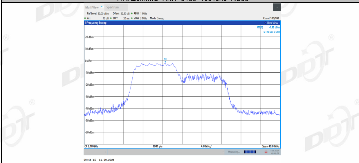
11AX20MIMO Ant1_5180_106Tone_RU54
