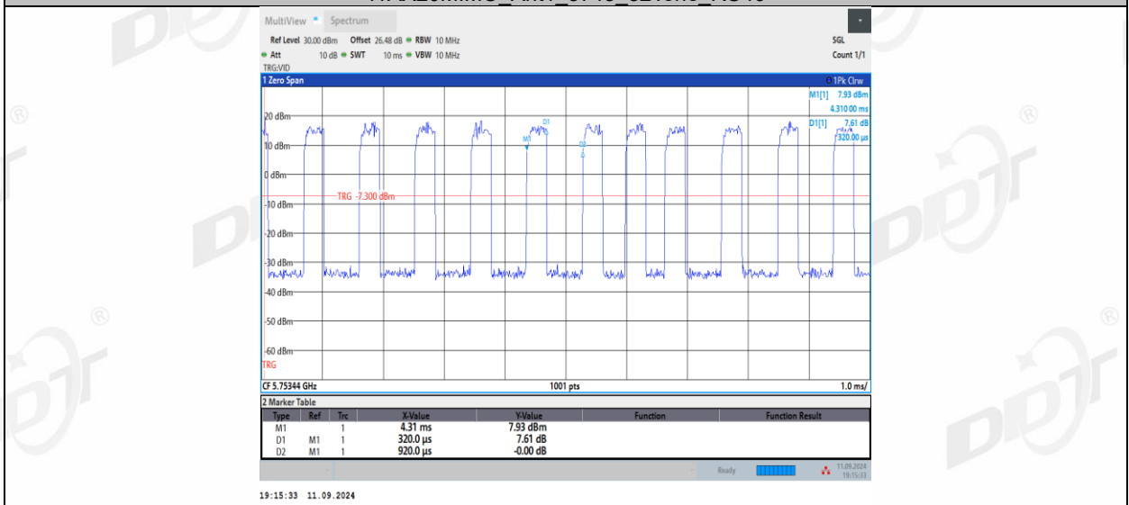
11AX20MIMO Ant1 5745_106Tone RU53
