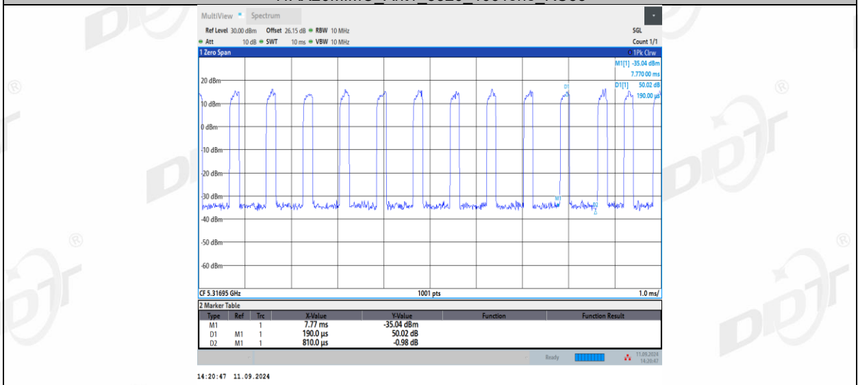
11AX20MIMO Ant1 5320_106Tone RU54
