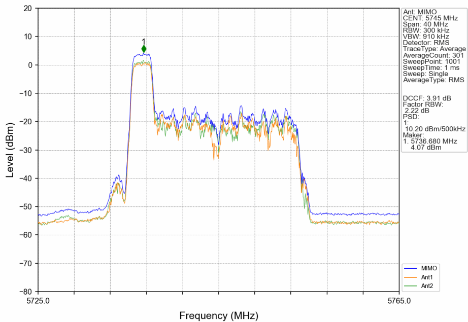
802.11ax(HEW20)_LCH_5745MHz_RU26_Left_MIMO_NTNV
