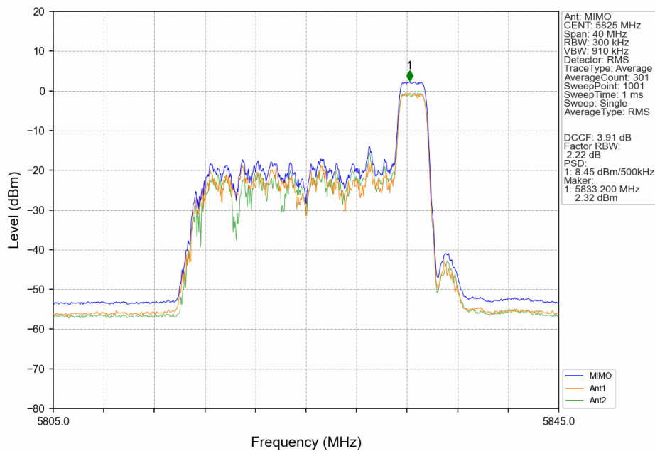
802.11ax(HEW20)_HCH_5825MHz_RU26_Right_MIMO_NTNV
