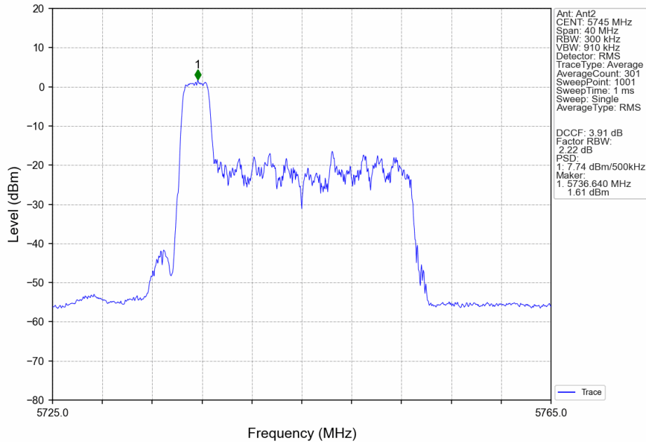
802.11ax(HEW20)_LCH_5745MHz_RU26_Left_MIMO_NTNV
