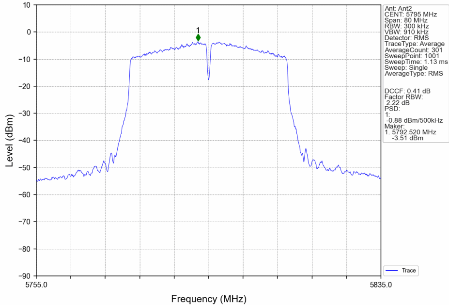
802.11ac(VHT40)_HCH_5795MHz_MIMO_NTNV
