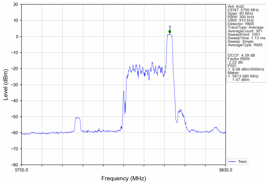
802.11ax(HEW40)_HCH_5795MHz_RU26_Right_MIMO_NTNV
