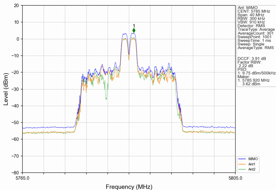
802.11ax(HEW20)_MCH_5785MHz_RU26_Mid_MIMO_NTNV
