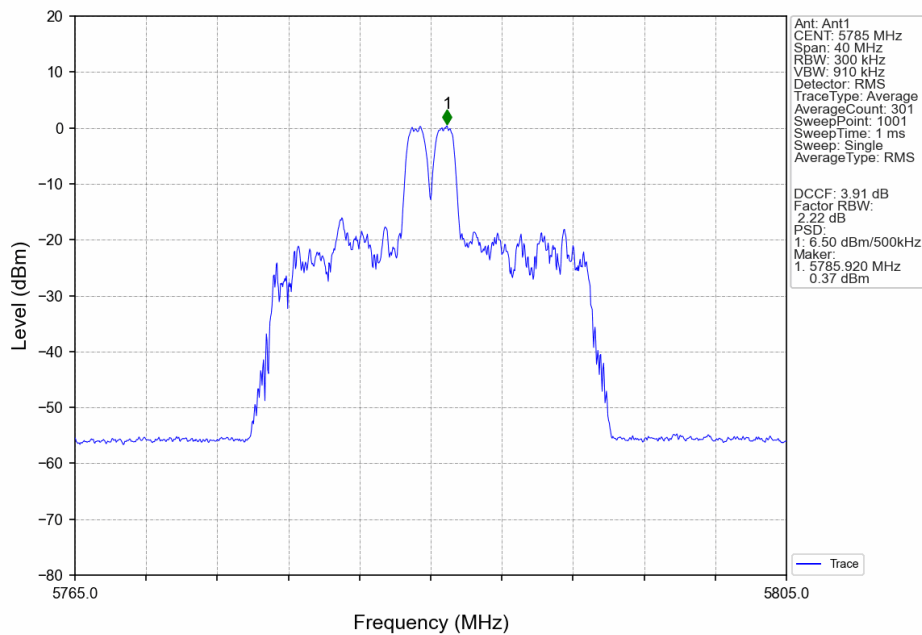
802.11ax(HEW20)_MCH_5785MHz_RU26_Mid_Ant1_NTNV
