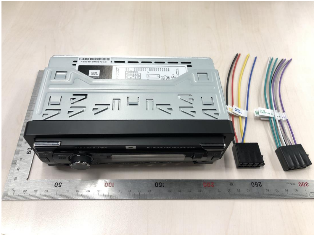
Fig. 1 External view
